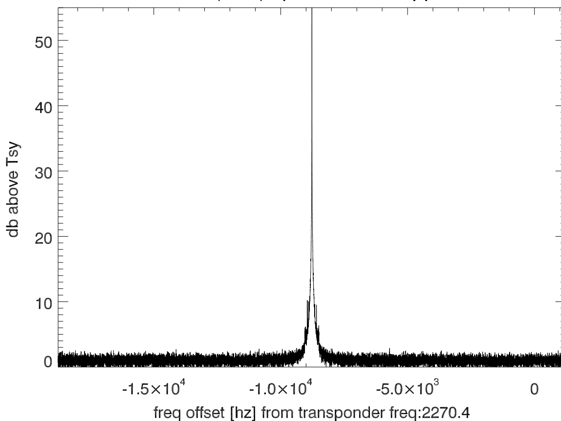
isee3 140620:182547 (UTC) spectra after doppler correction. PolB
