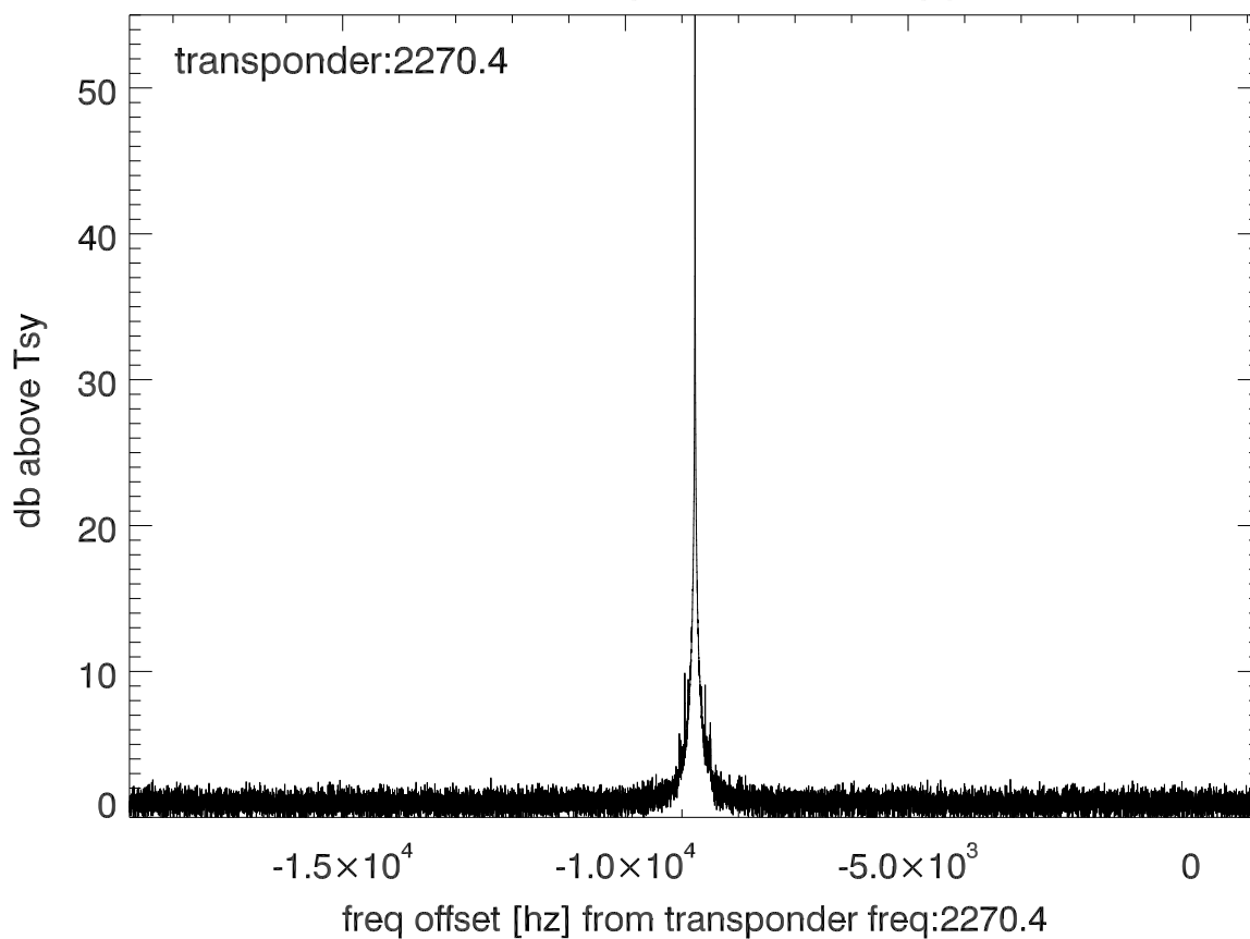
isee3 140620:182547 (UTC) spectra after doppler correction. PolA
