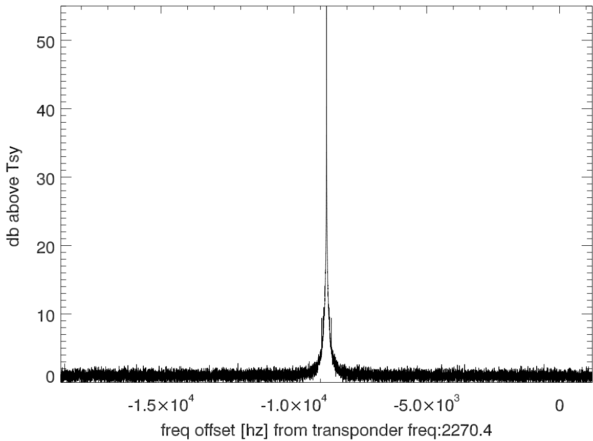
isee3 140620:181520 (UTC) spectra after doppler correction. PolB
