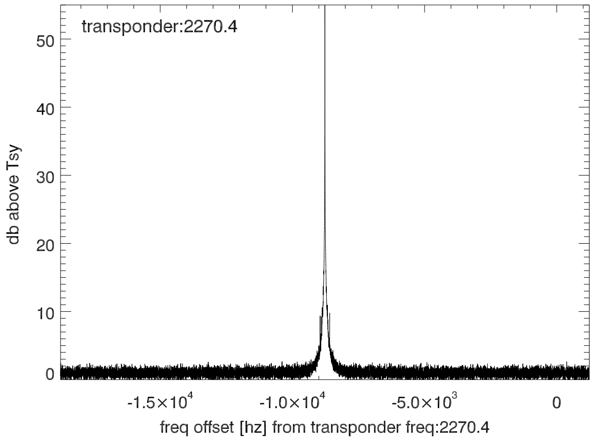
isee3 140620:181520 (UTC) spectra after doppler correction. PolA
