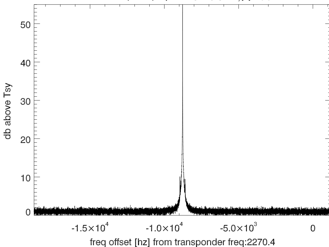
isee3 140620:175717 (UTC) spectra after doppler correction. PolB
