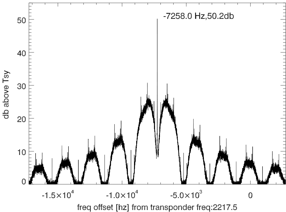
isee3 140620:193245 (UTC) spectra after doppler correction. PoIB
