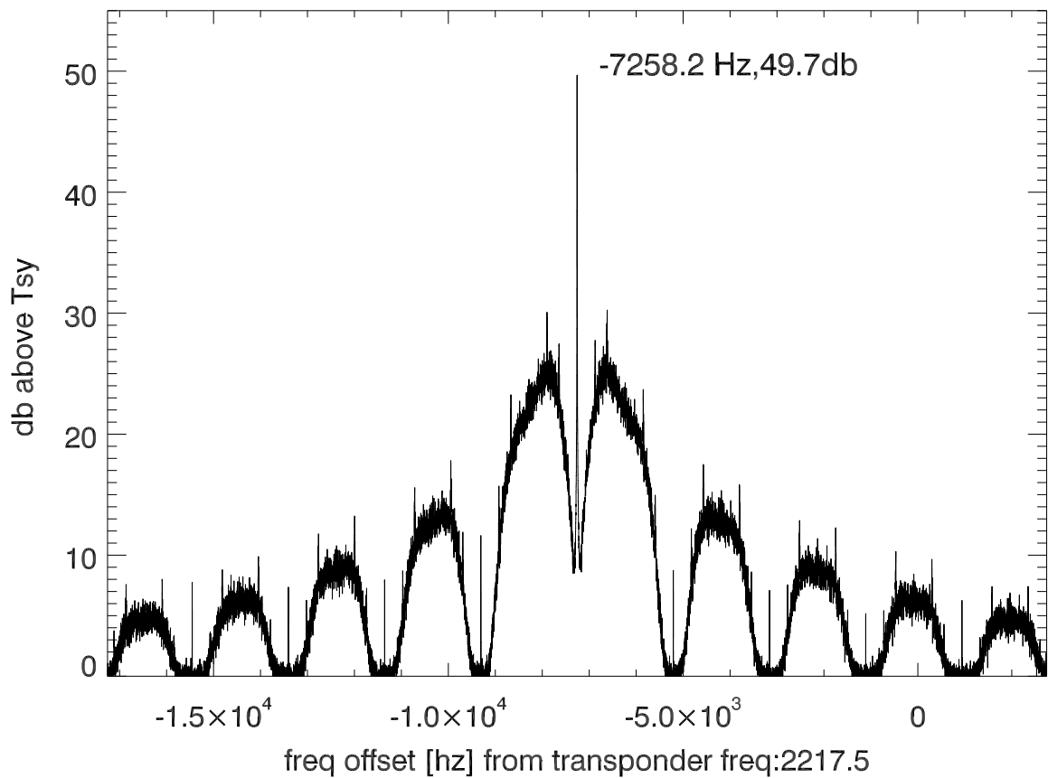
isee3 140620:192010 (UTC) spectra after doppler correction. PoIB
