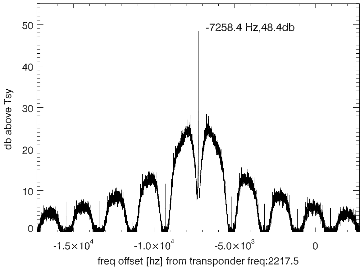
isee3 140620:190752 (UTC) spectra after doppler correction. PolB
