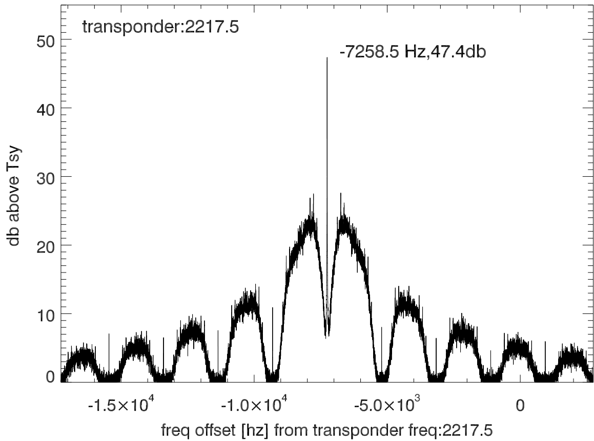
isee3 140620:190752 (UTC) spectra after doppler correction. PolA
