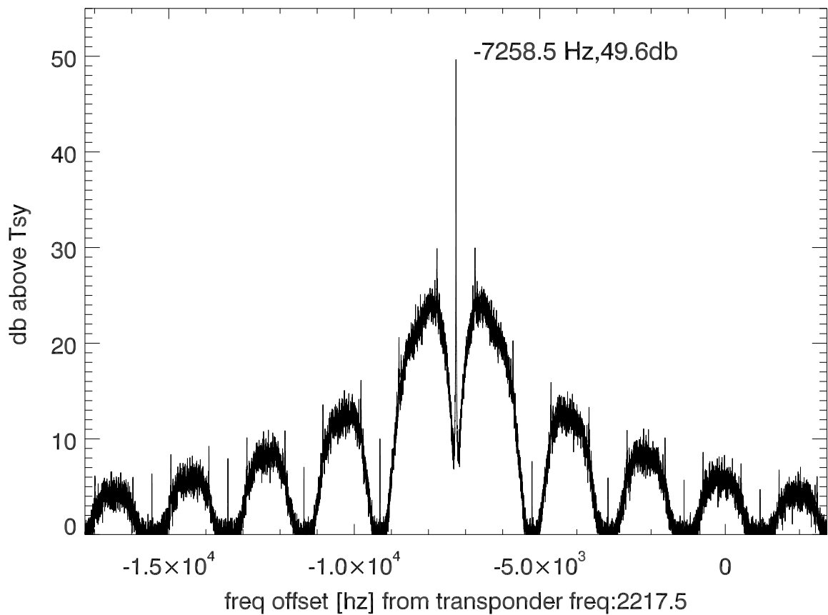
isee3 140620:190337 (UTC) spectra after doppler correction. PoIB
