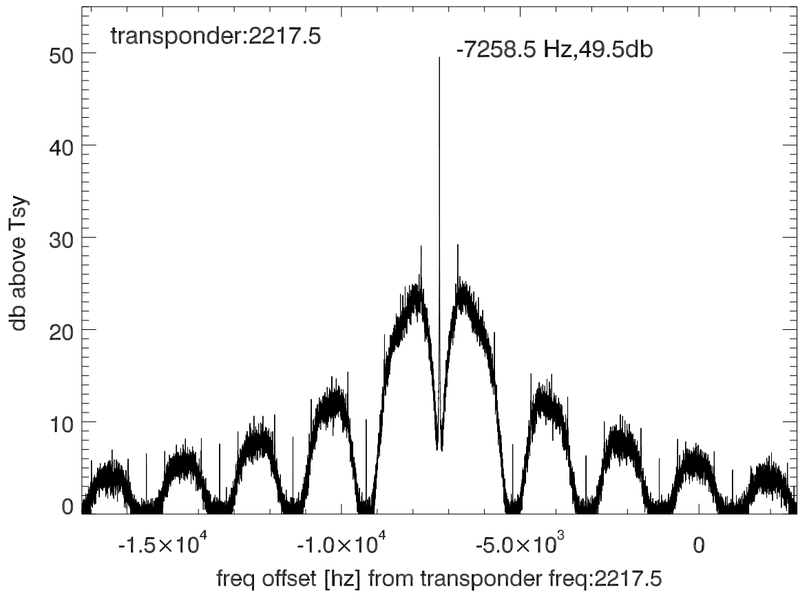
isee3 140620:190337 (UTC) spectra after doppler correction. PoIA
