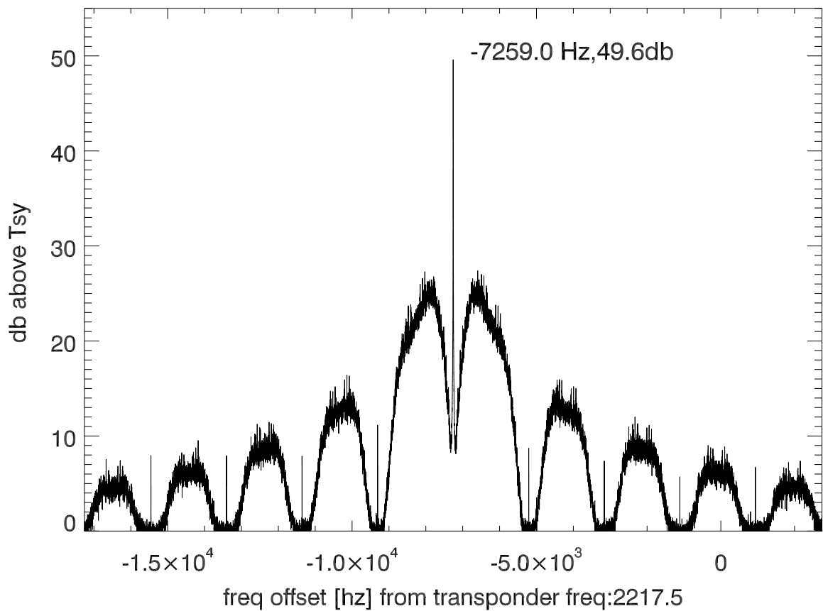
isee3 140620:184328 (UTC) spectra after doppler correction. PoIB
