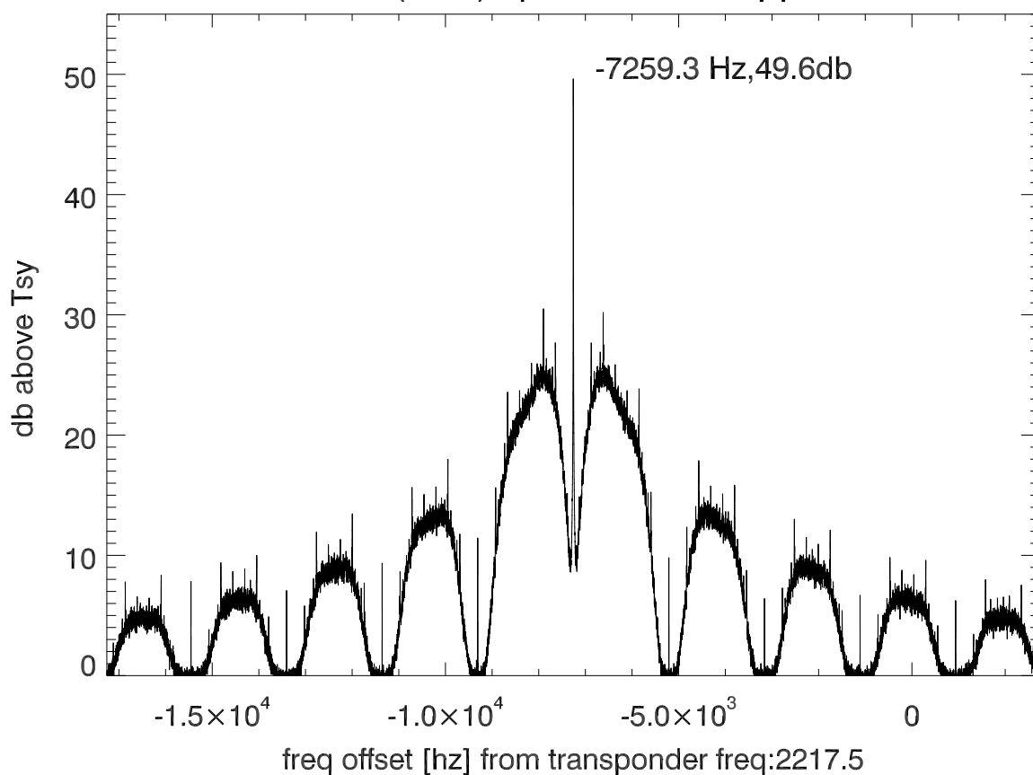
isee3 140620:183349 (UTC) spectra after doppler correction. PoIB
