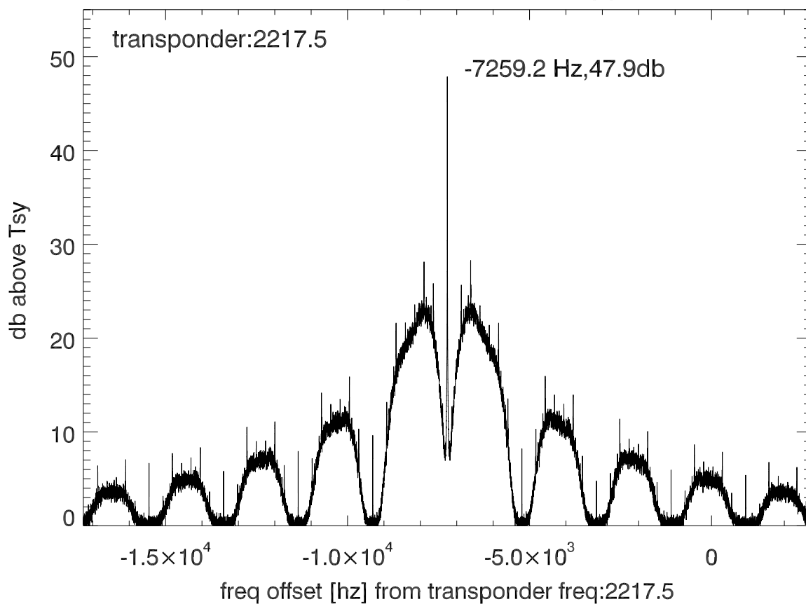
isee3 140620:183349 (UTC) spectra after doppler correction. PoIA
