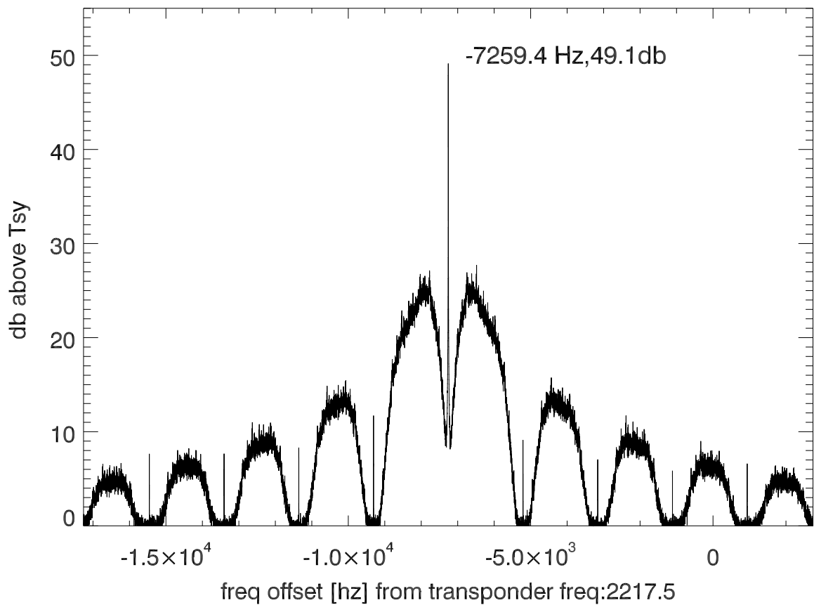
isee3 140620:182547 (UTC) spectra after doppler correction. PoIB
