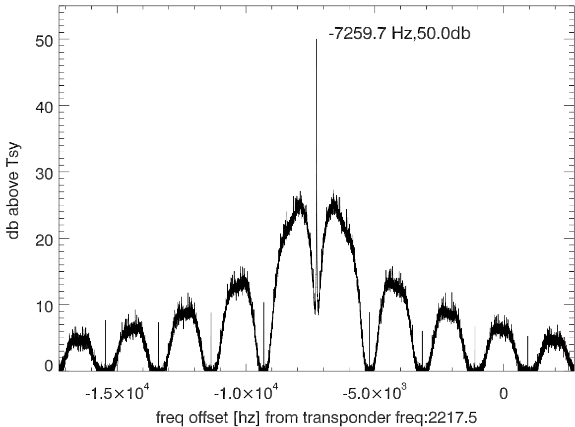
isee3 140620:181520 (UTC) spectra after doppler correction. PoIB
