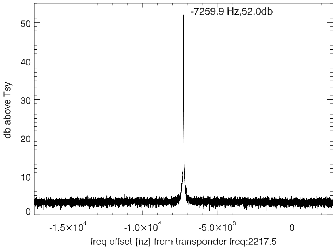
isee3 140620:180117 (UTC) spectra after doppler correction. PolB
