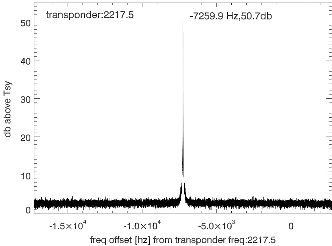
isee3 140620:180117 (UTC) spectra after doppler correction. PolA
