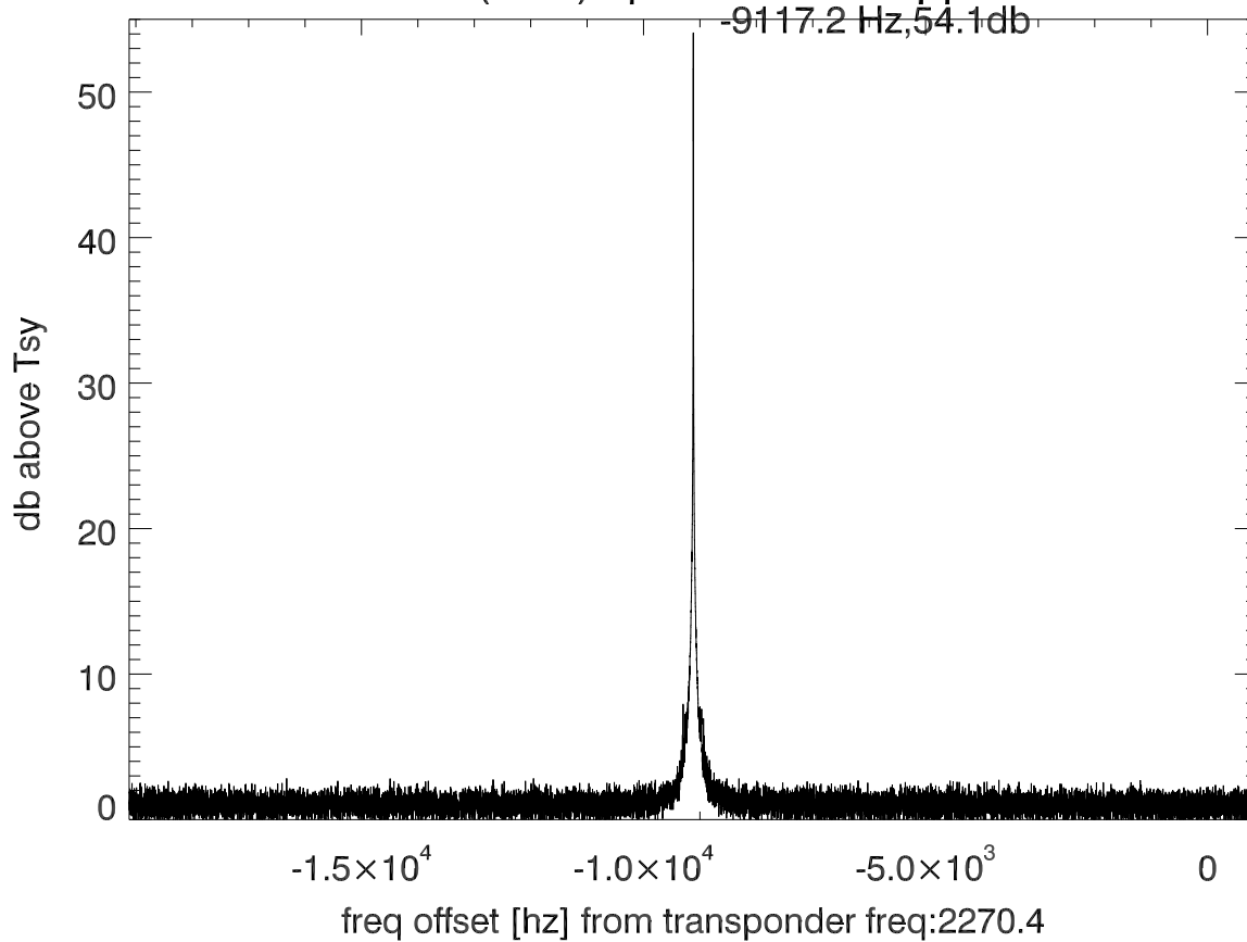
isee3 140615:191428 (UTC) spectra after doppler correction. PoIB
