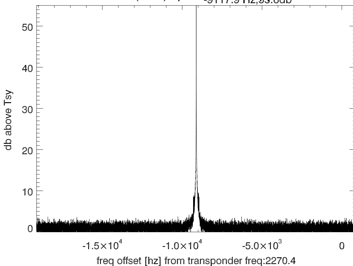
isee3 140615:190400 (UTC) spectra after doppler correction. PolB
