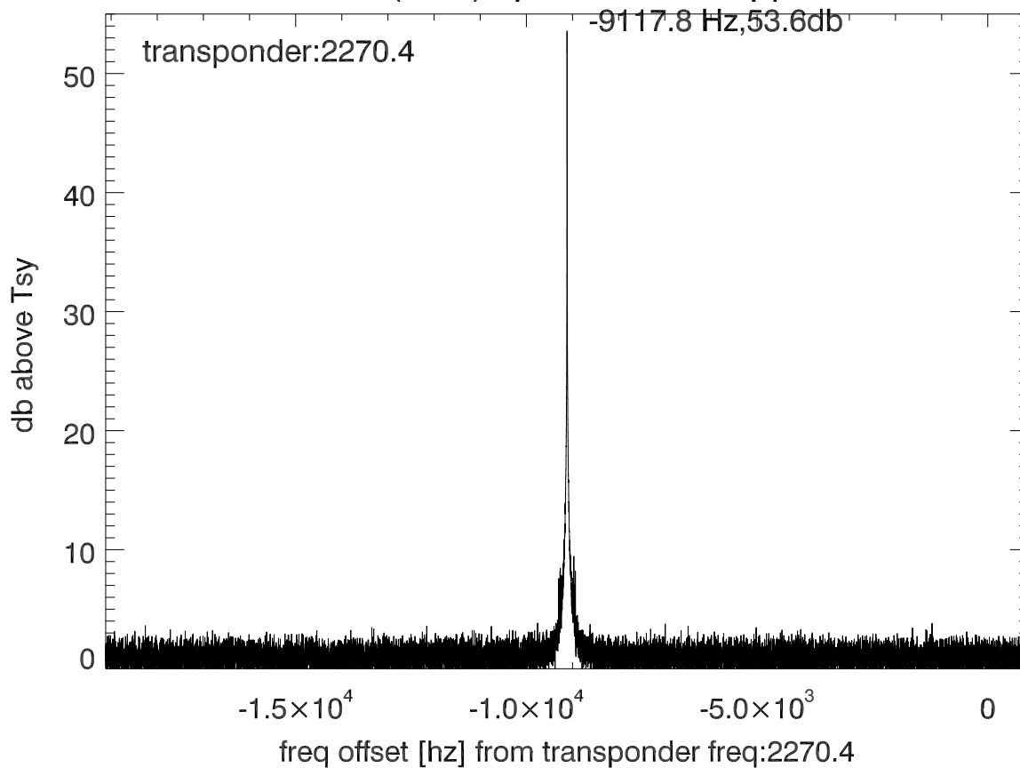
isee3 140615:190400 (UTC) spectra after doppler correction. PolA
