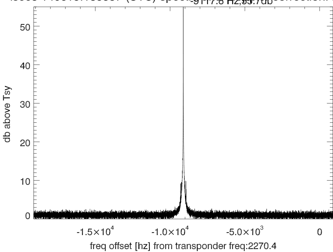
isee3 140615:185337 (UTC) spectra after doppler correction. PolB
