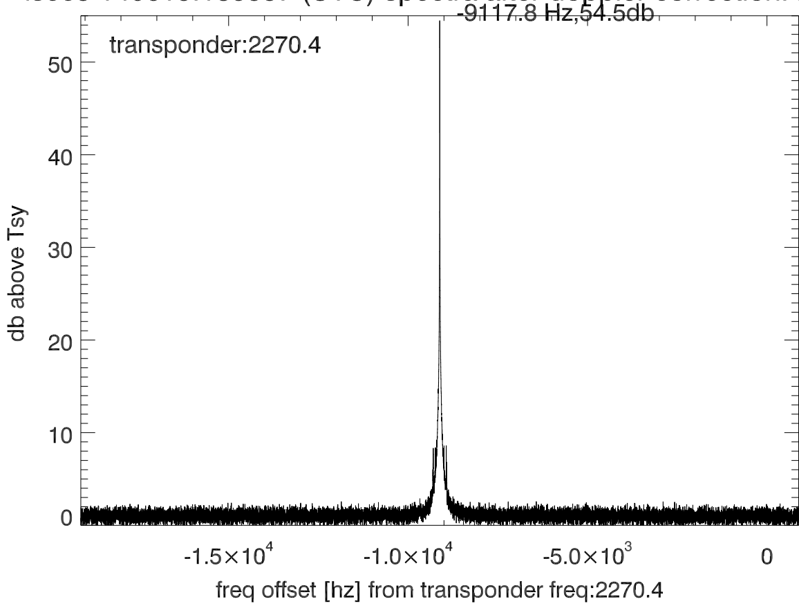
isee3 140615:185337 (UTC) spectra after doppler correction. PolA
