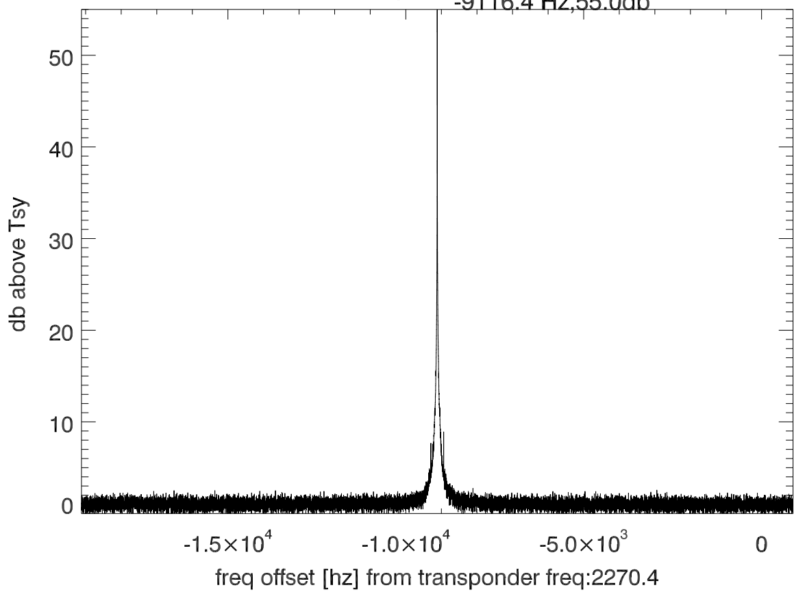
isee3 140615:193900 (UTC) spectra after doppler correction. PoIB
