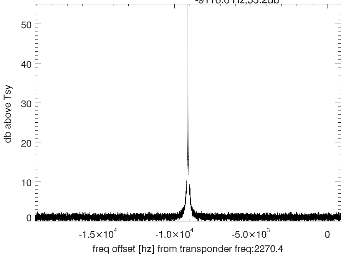
isee3 140615:193544 (UTC) spectra after doppler correction. PoIB
