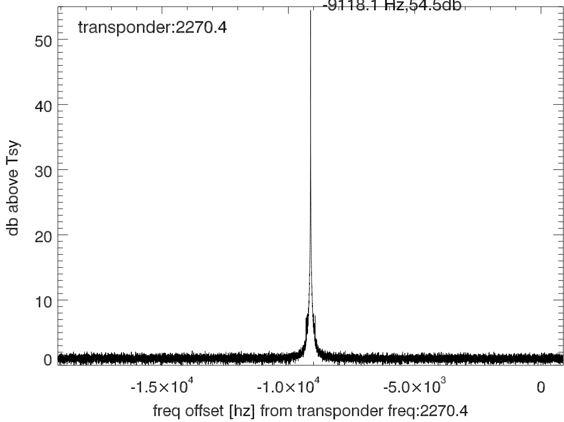
isee3 140615:184453 (UTC) spectra after doppler correction. PolA
