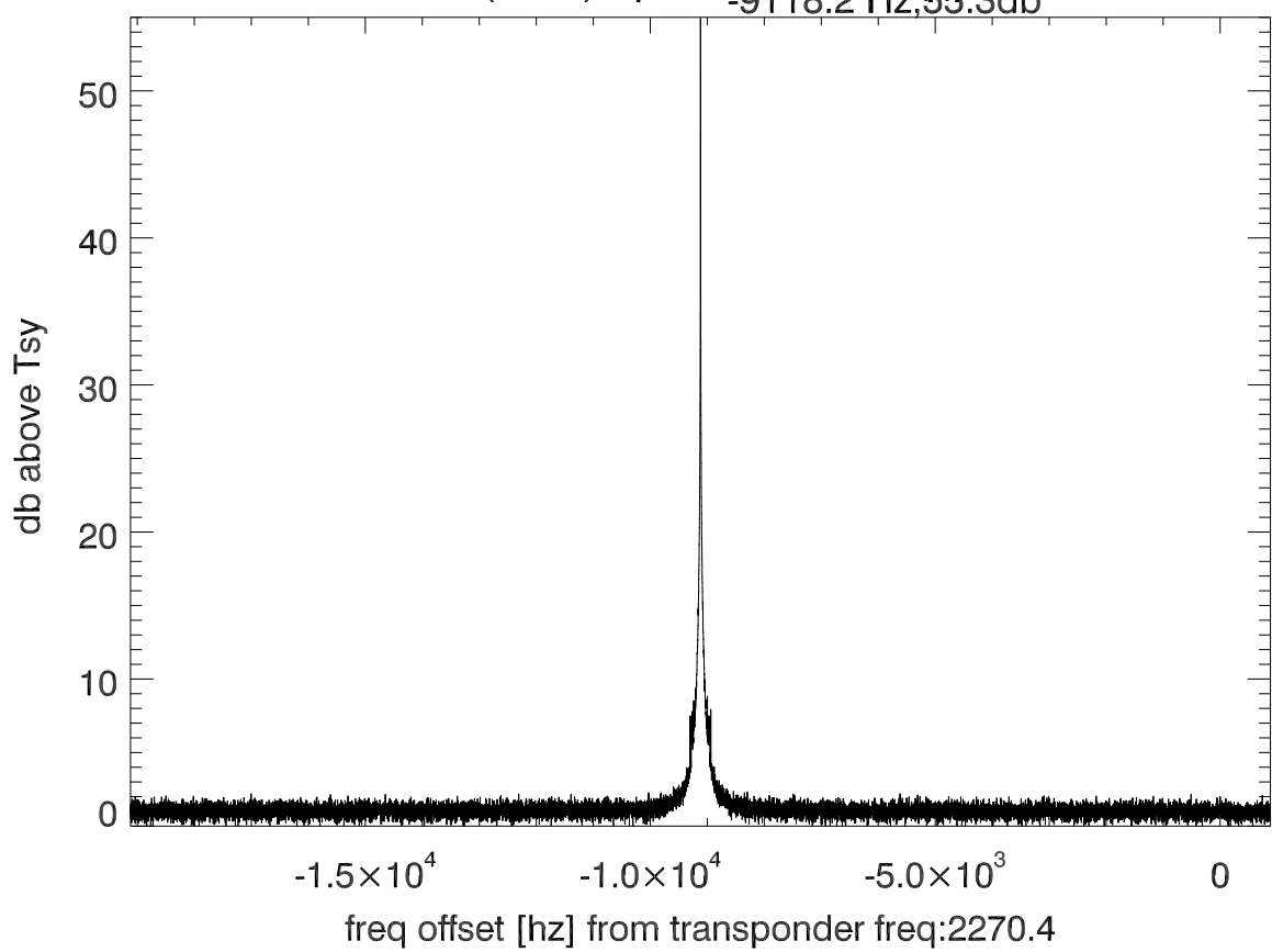
isee3 140615:184453 (UTC) spectra after doppler correction. PolB
