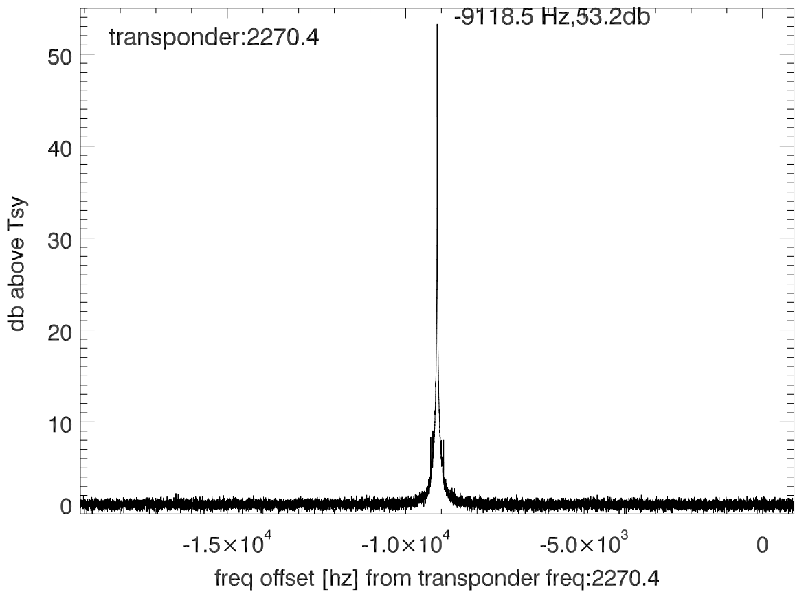
isee3 140615:184004 (UTC) spectra after doppler correction. PolA
