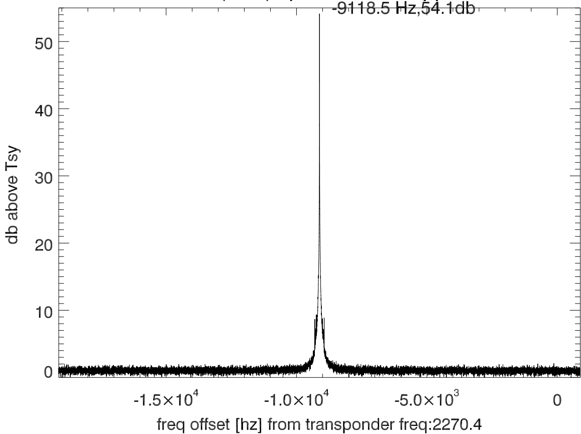
isee3 140615:184004 (UTC) spectra after doppler correction. PolB
