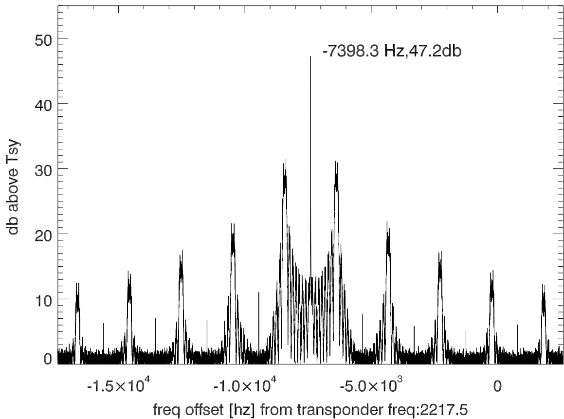
isee3 140615:190641 (UTC) spectra after doppler correction. PoIB
