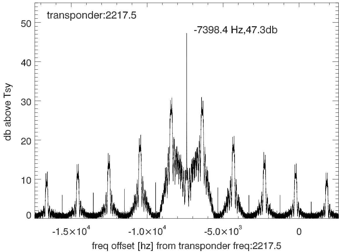
isee3 140615:185828 (UTC) spectra after doppler correction. PoIA
