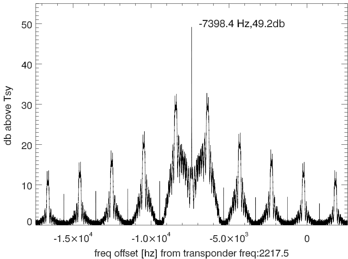
isee3 140615:185828 (UTC) spectra after doppler correction. PoIB
