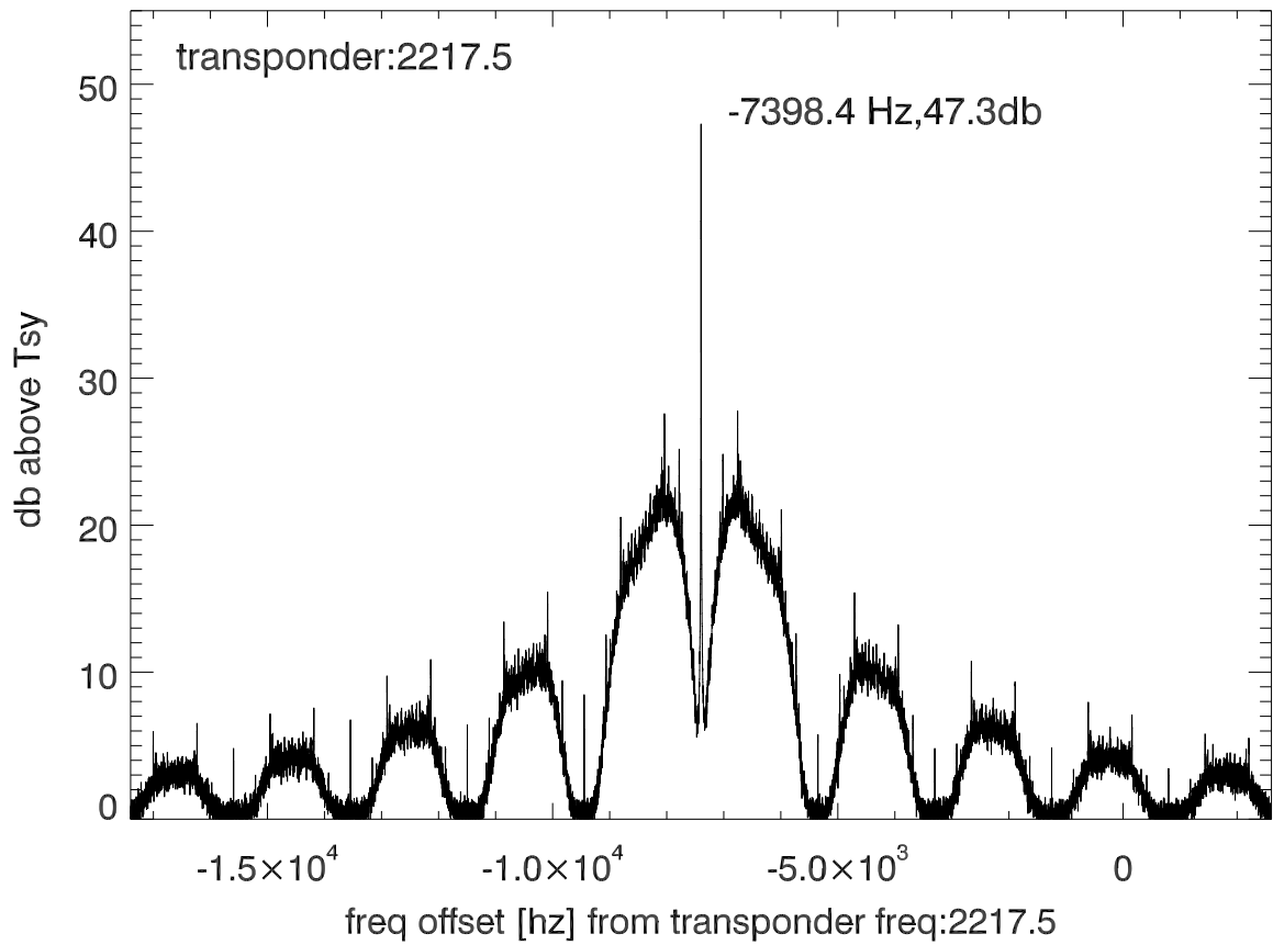
isee3 140615:185337 (UTC) spectra after doppler correction. PoIA
