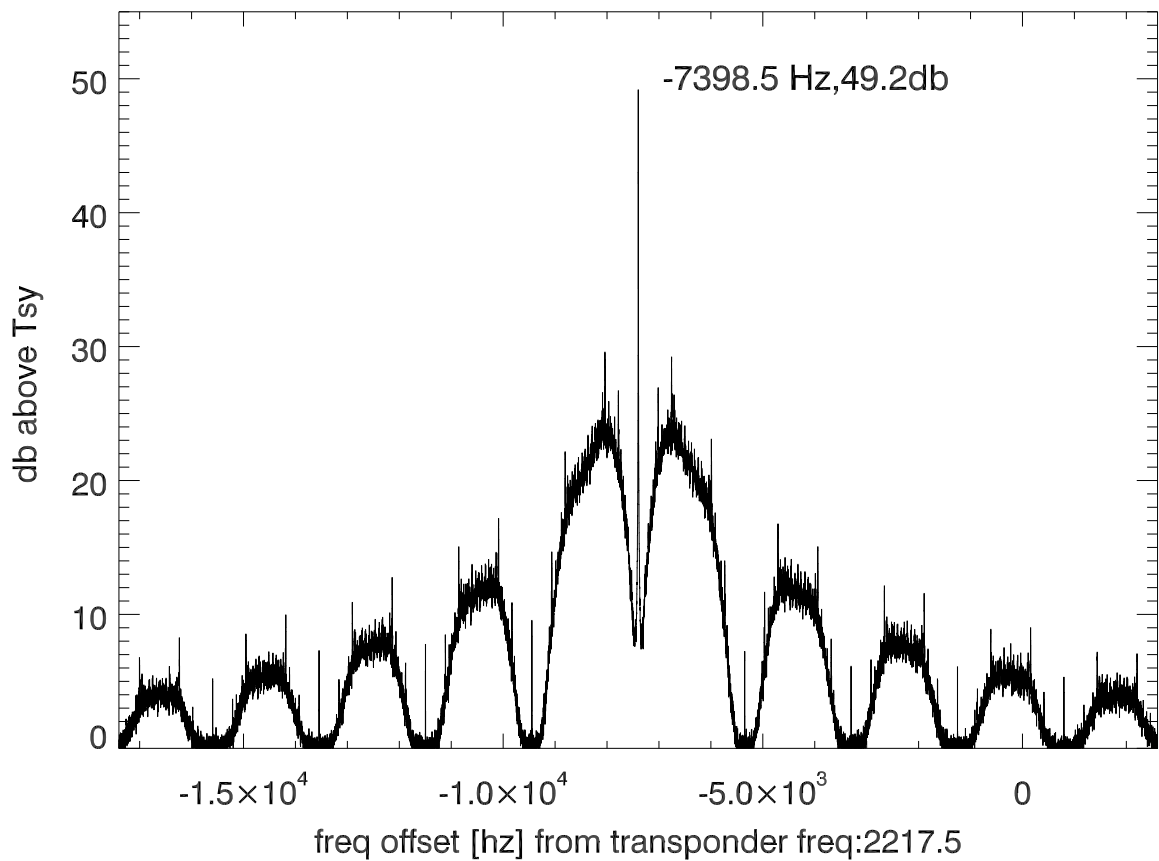
isee3 140615:185337 (UTC) spectra after doppler correction. PoIB
