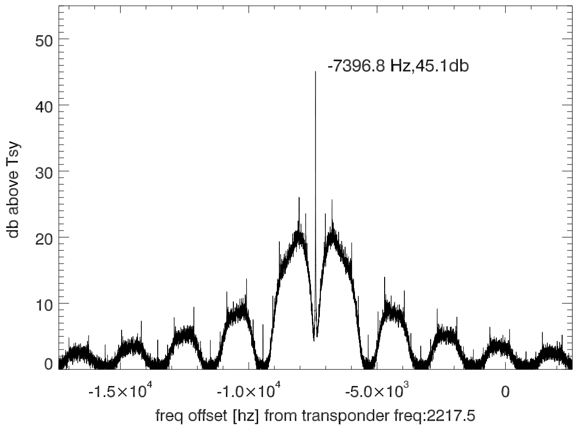
isee3 140615:202918 (UTC) spectra after doppler correction. PolB
