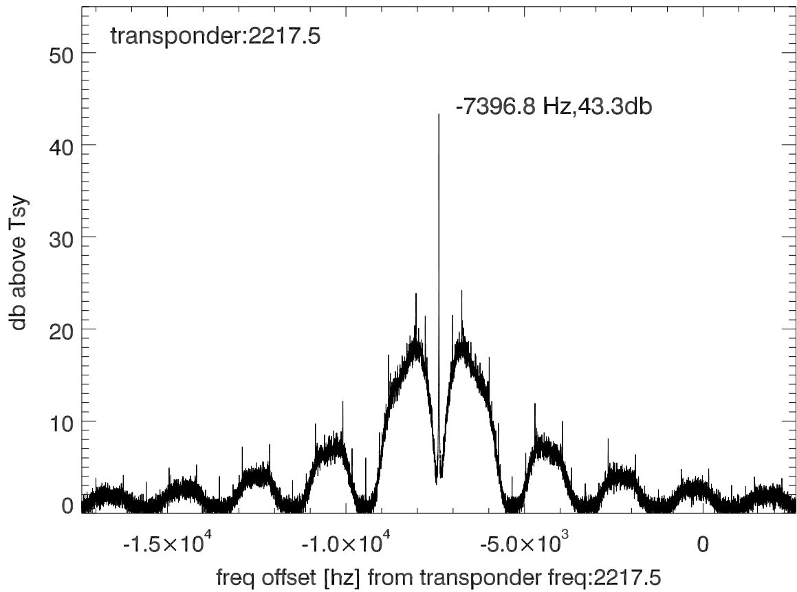
isee3 140615:202918 (UTC) spectra after doppler correction. PolA
