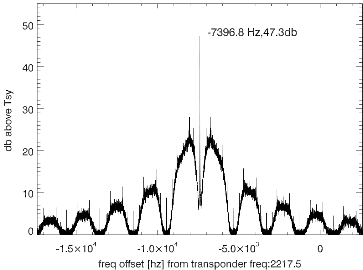
isee3 140615:202301 (UTC) spectra after doppler correction. PoIB
