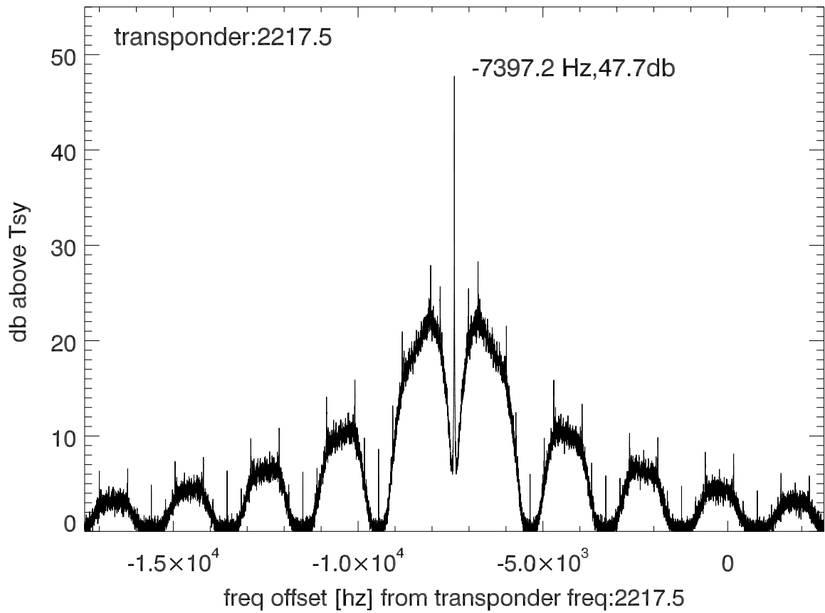
isee3 140615:200719 (UTC) spectra after doppler correction. PolA
