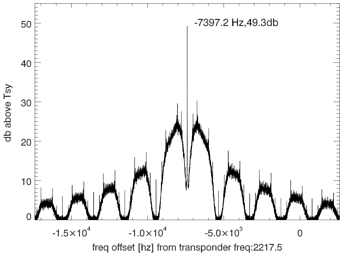
isee3 140615:200719 (UTC) spectra after doppler correction. PolB
