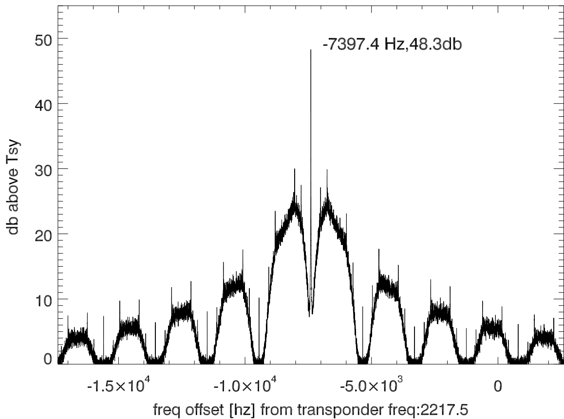
isee3 140615:195434 (UTC) spectra after doppler correction. PolB
