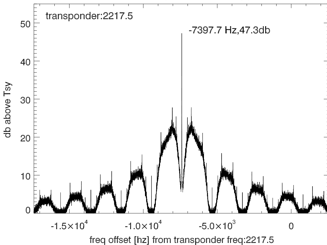
isee3 140615:194159 (UTC) spectra after doppler correction. PolA
