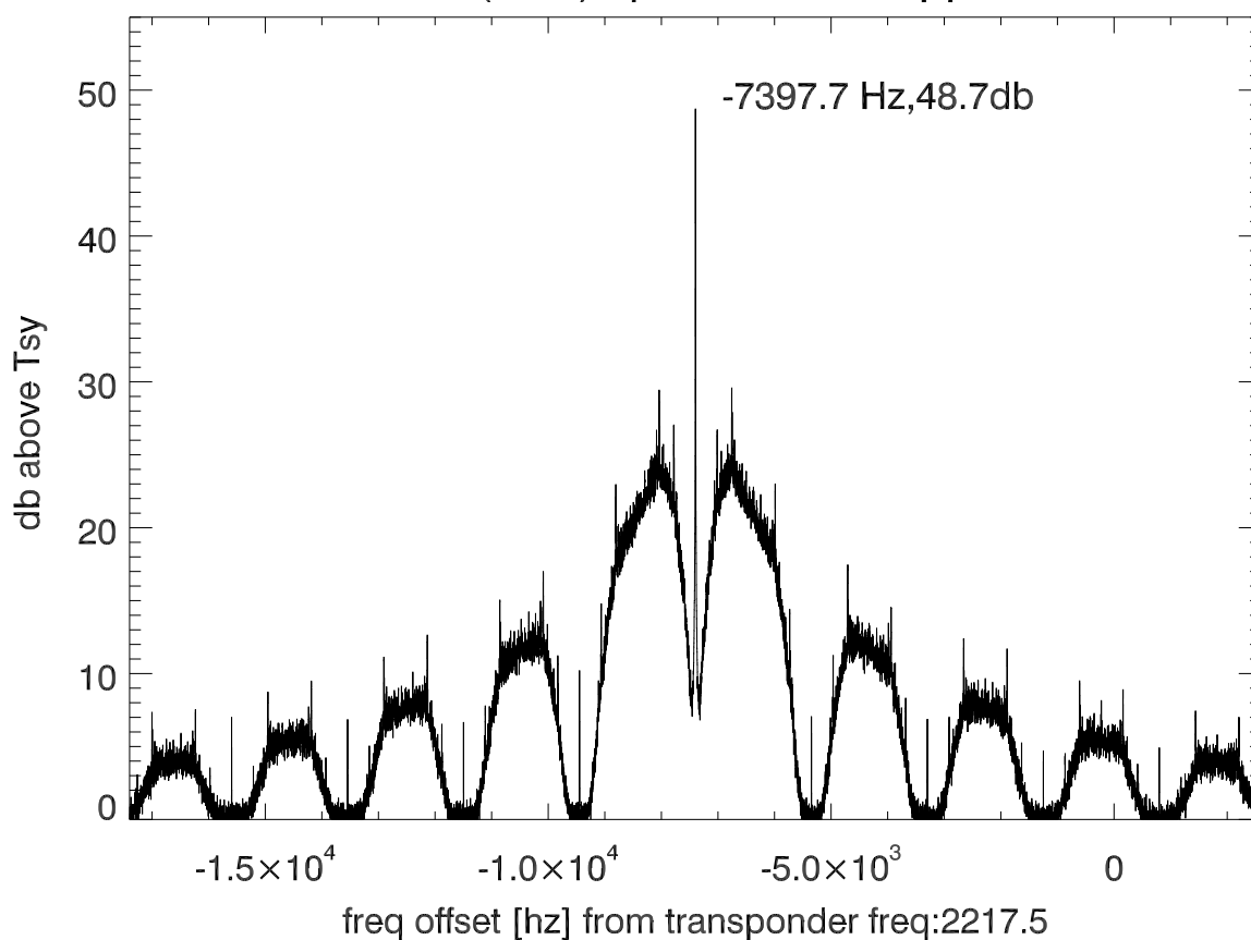
isee3 140615:194159 (UTC) spectra after doppler correction. PolB
