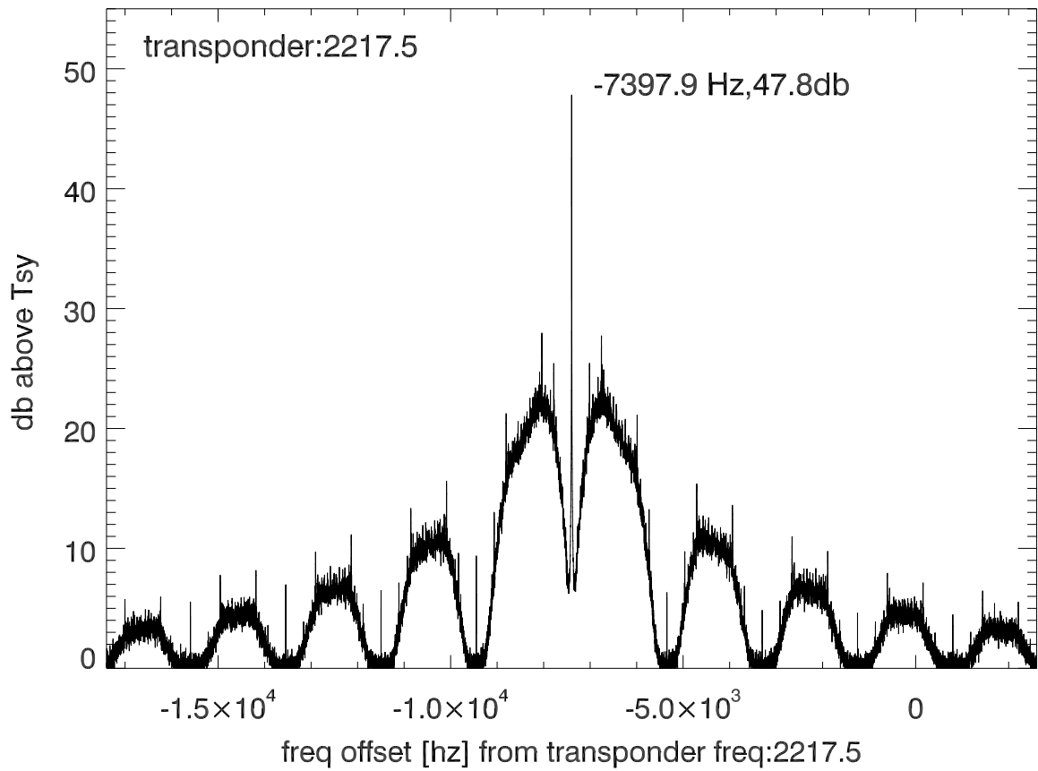
isee3 140615:193224 (UTC) spectra after doppler correction. PolA
