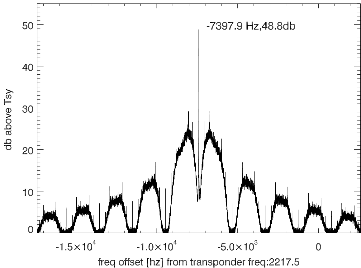
isee3 140615:193224 (UTC) spectra after doppler correction. PolB
