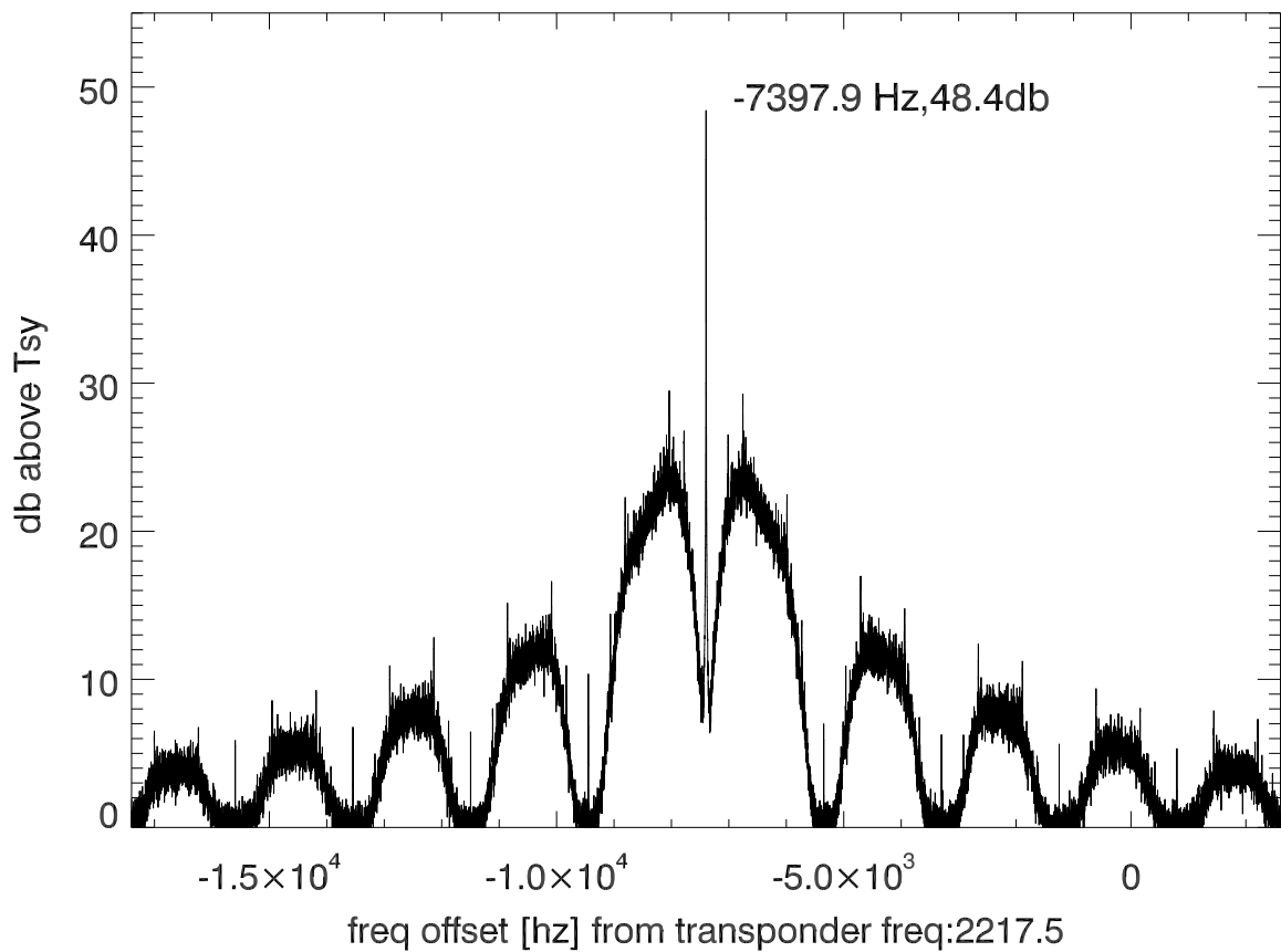
isee3 140615:192426 (UTC) spectra after doppler correction. PoIB
