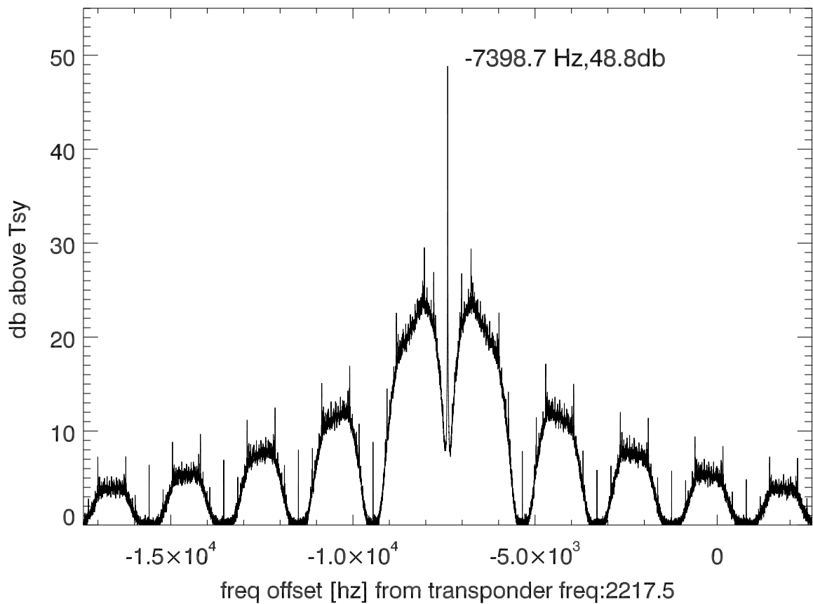
isee3 140615:184004 (UTC) spectra after doppler correction. PoIB
