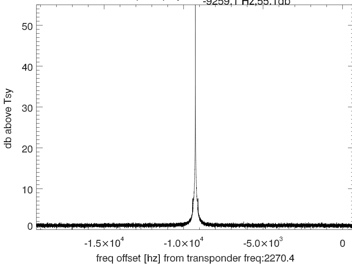
isee3 140613:201909 (UTC) spectra after doppler correction. PolB
