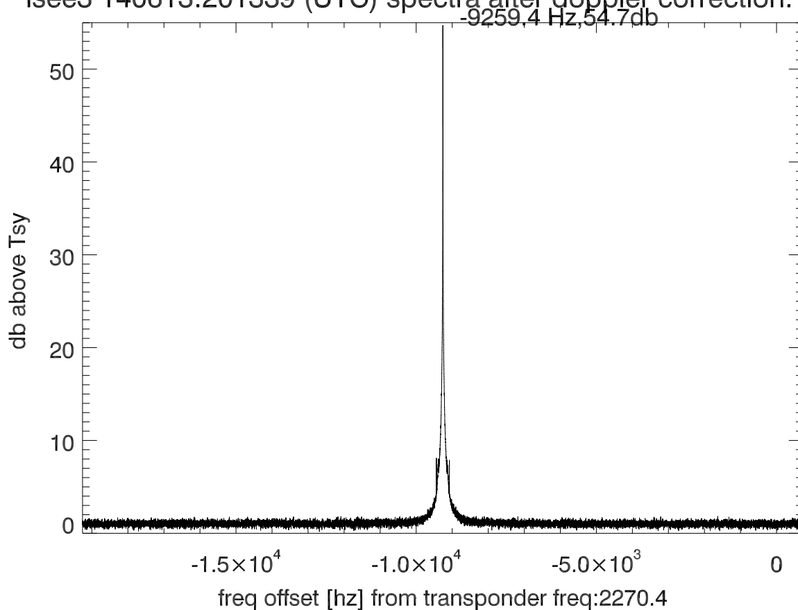
isee3 140613:201339 (UTC) spectra after doppler correction. PolB
