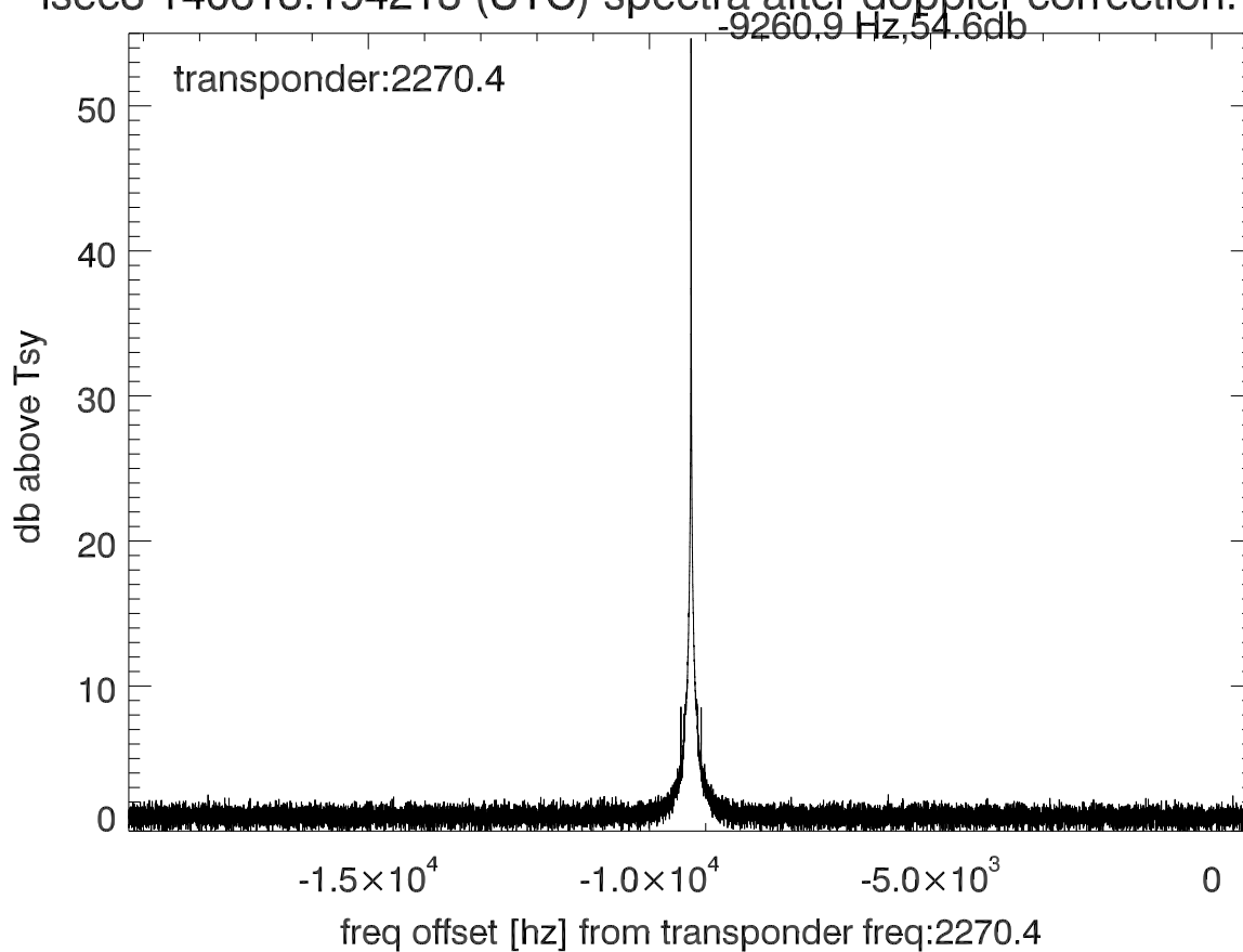
isee3 140613:194218 (UTC) spectra after doppler correction. PolA
