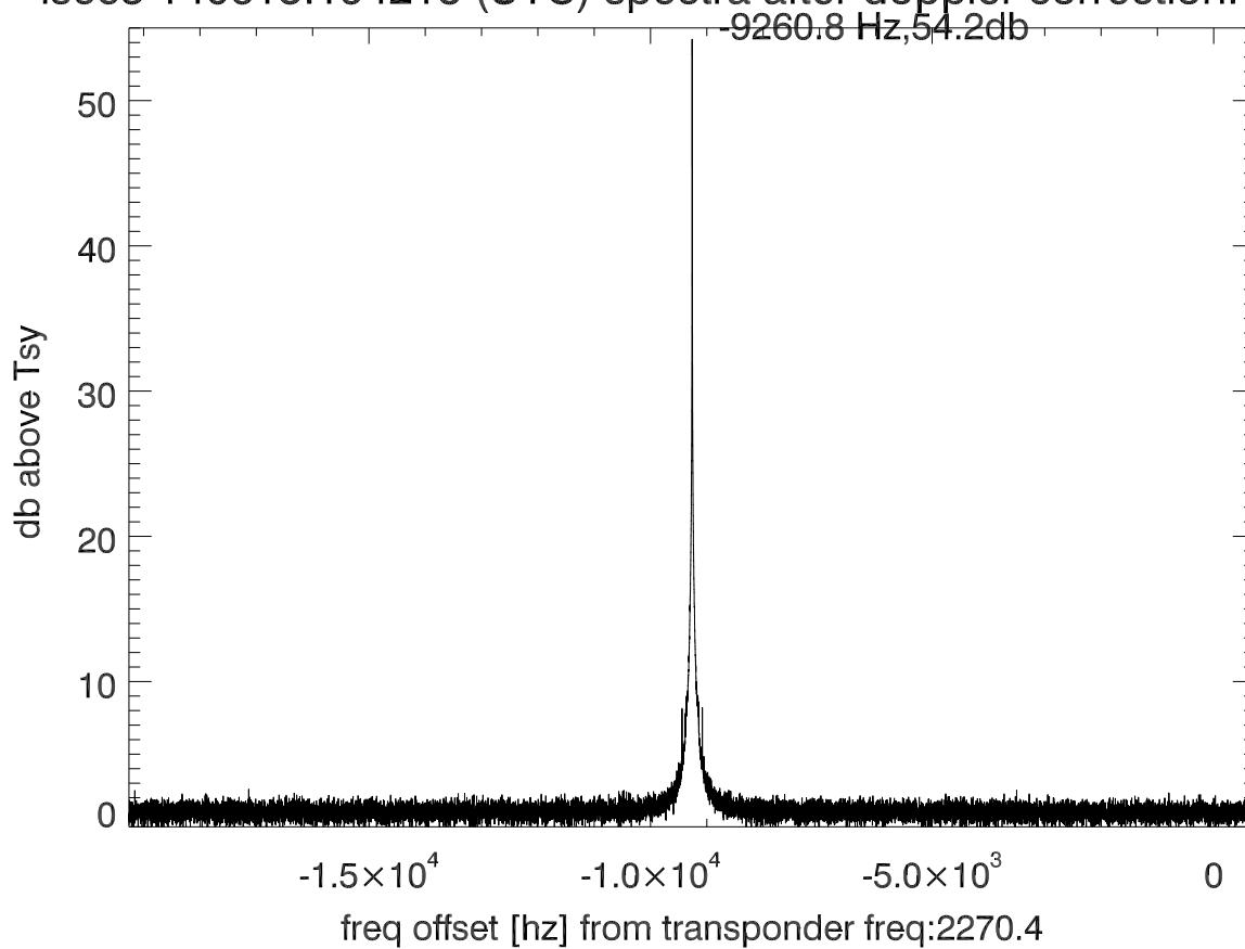
isee3 140613:194218 (UTC) spectra after doppler correction. PolB
