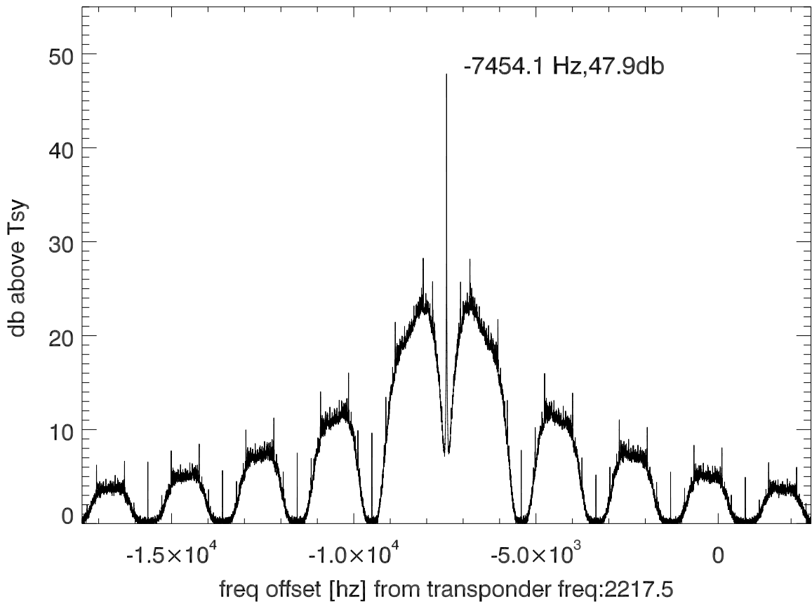
isee3 140613:202450 (UTC) spectra after doppler correction. PolB
