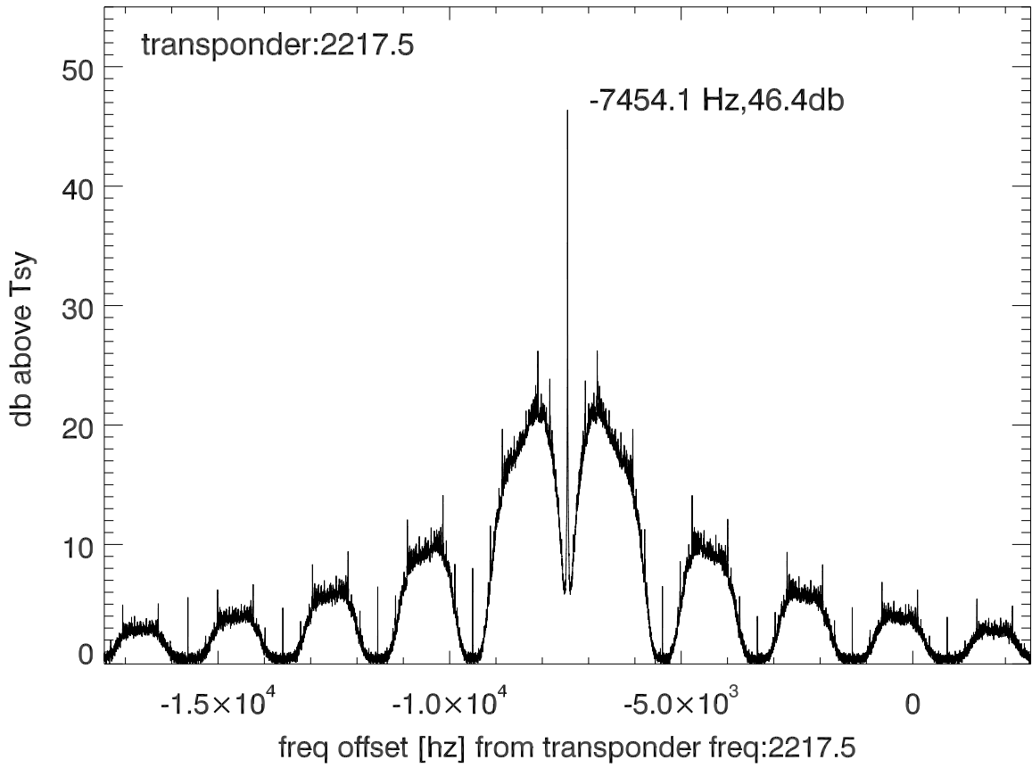
isee3 140613:202450 (UTC) spectra after doppler correction. PolA
