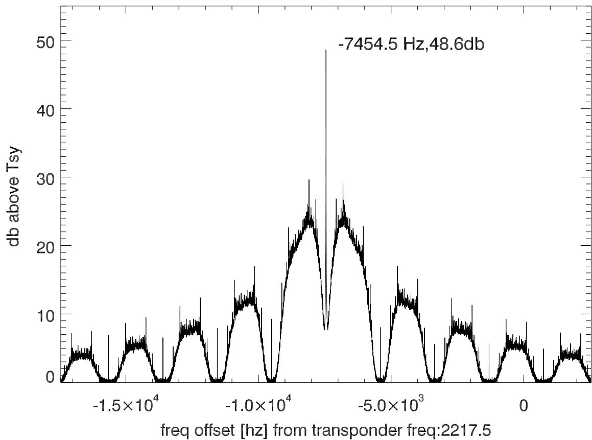
isee3 140613:200649 (UTC) spectra after doppler correction. PoIB
