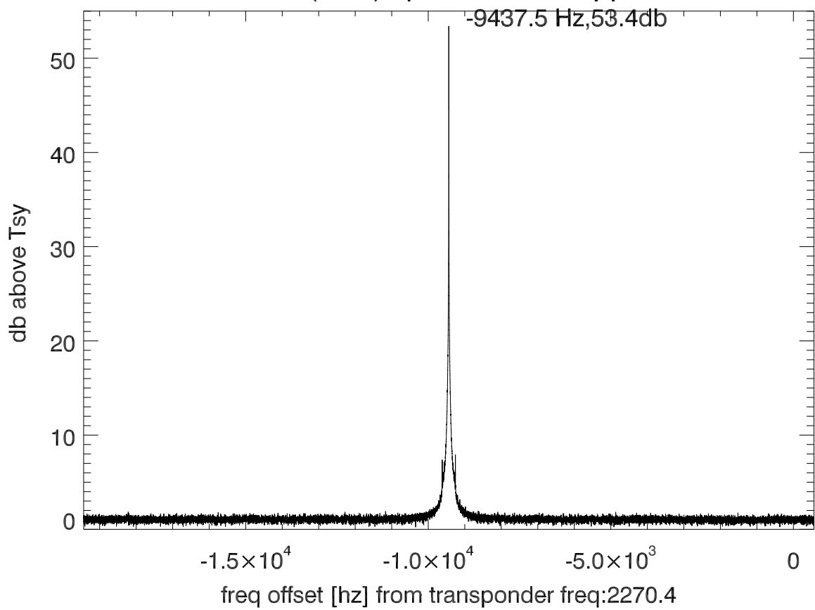
isee3 140610:195222 (UTC) spectra after doppler correction. PolB
