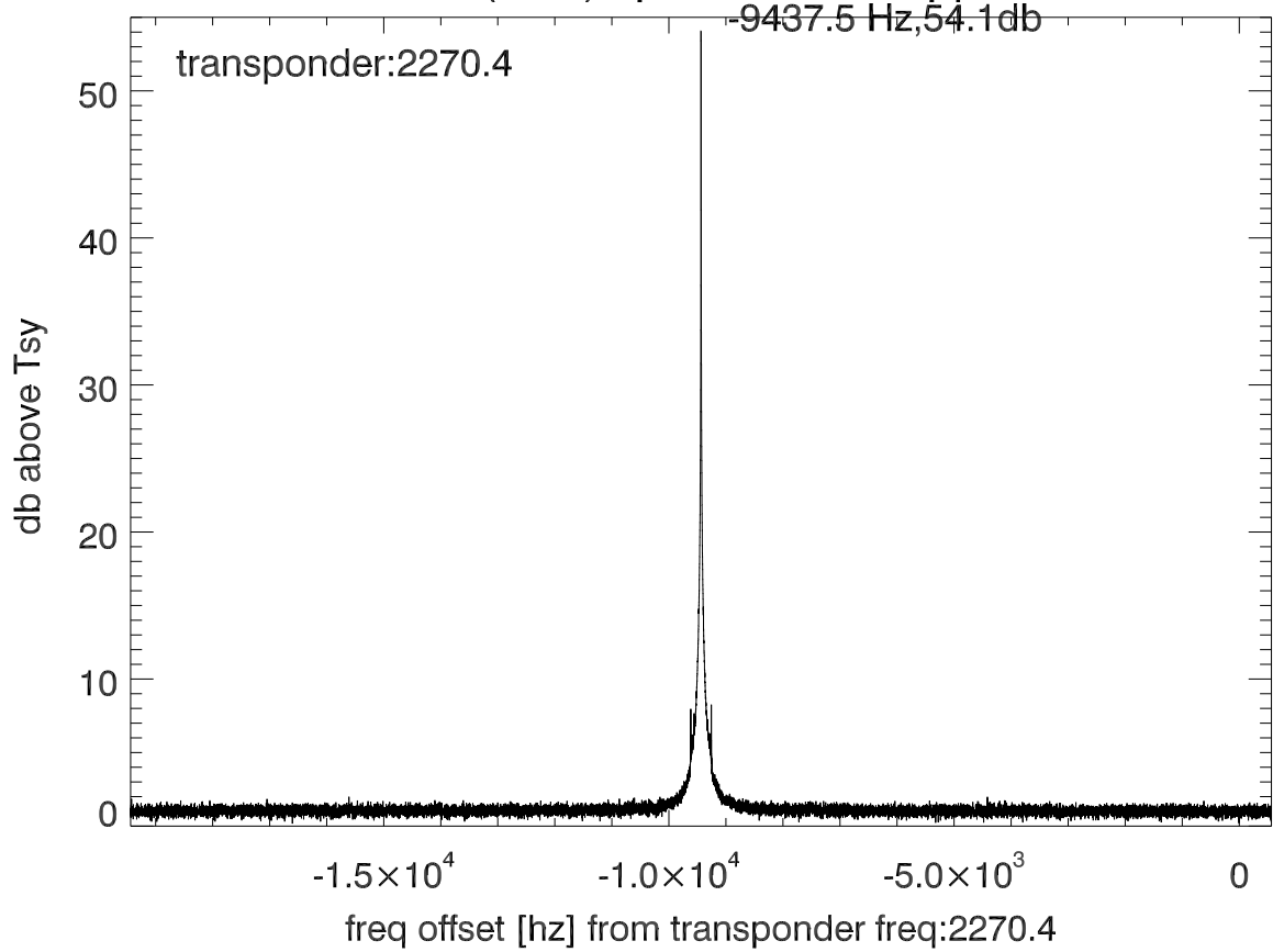
isee3 140610:195222 (UTC) spectra after doppler correction. PolA
