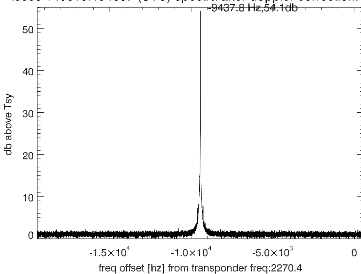
isee3 140610:194607 (UTC) spectra after doppler correction. PoIB
