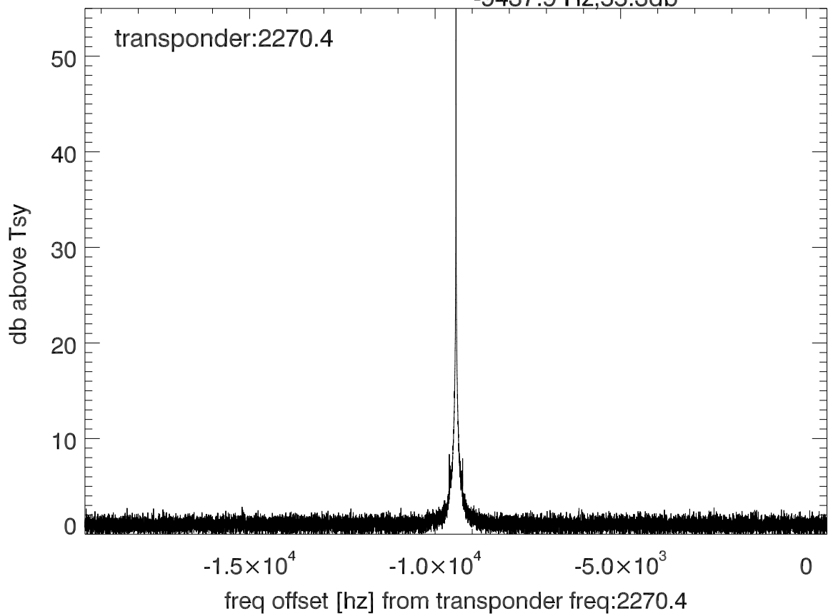
isee3 140610:194412 (UTC) spectra after doppler correction. PolA
