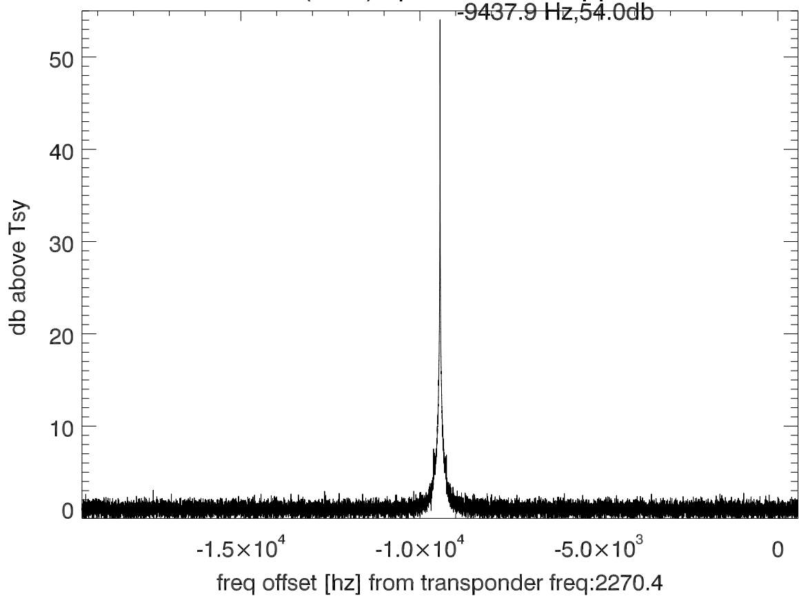
isee3 140610:194412 (UTC) spectra after doppler correction. PolB
