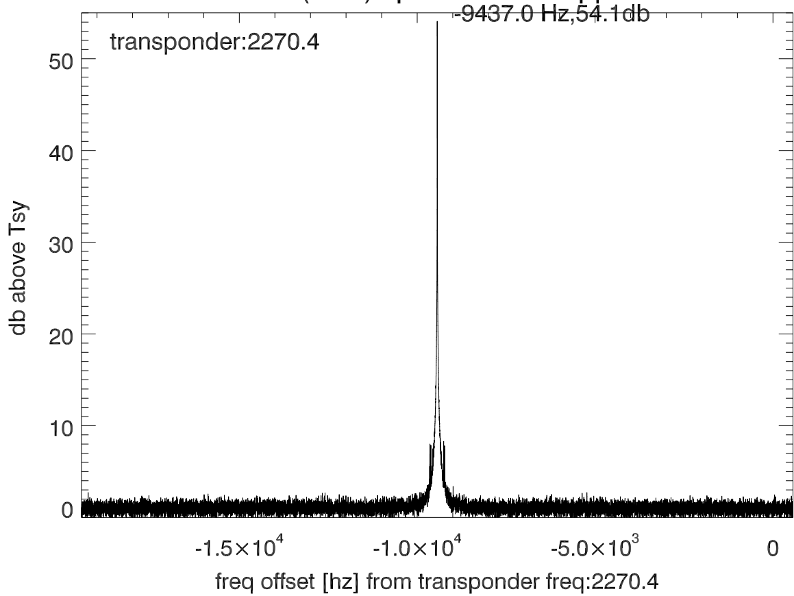
isee3 140610:202708 (UTC) spectra after doppler correction. PolA
