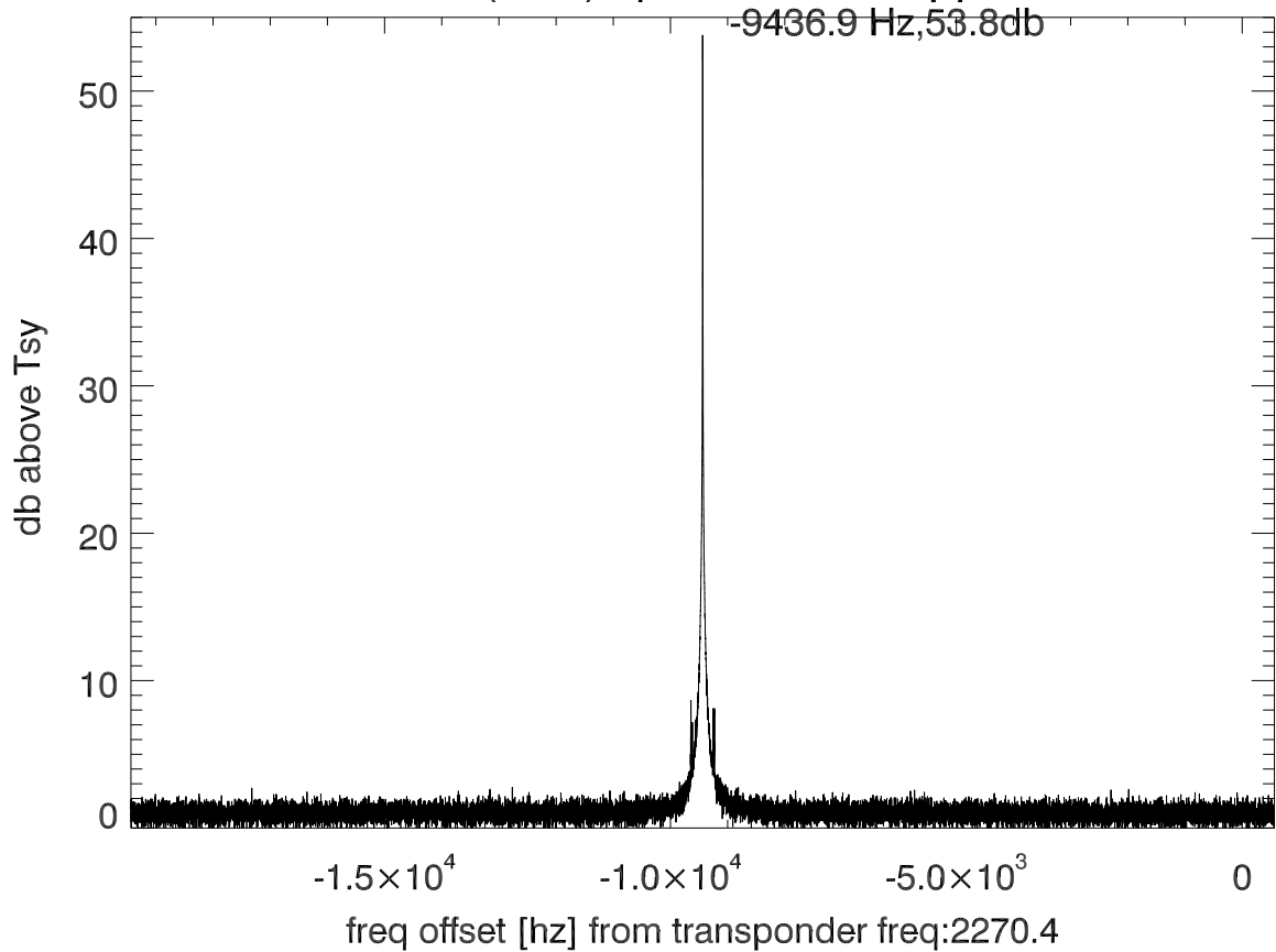
isee3 140610:202708 (UTC) spectra after doppler correction. PolB
