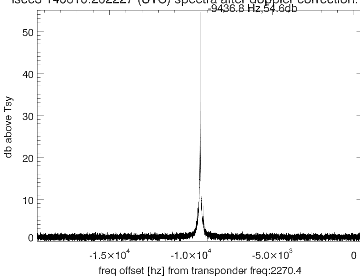
isee3 140610:202227 (UTC) spectra after doppler correction. PolB
