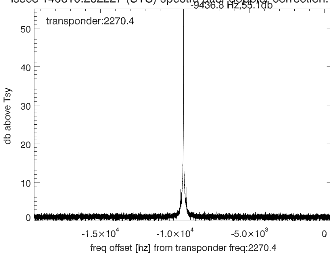
isee3 140610:202227 (UTC) spectra after doppler correction. PolA
