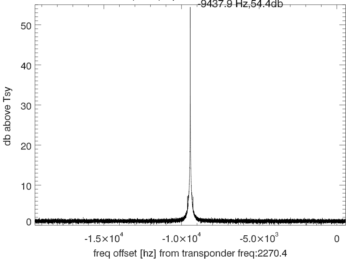
isee3 140610:193553 (UTC) spectra after doppler correction. PoIB
