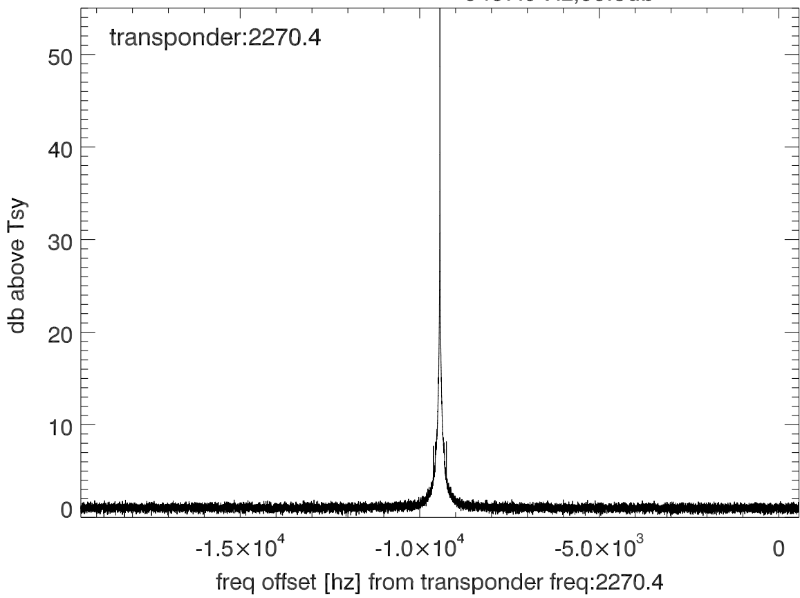
isee3 140610:193553 (UTC) spectra after doppler correction. PoIA
