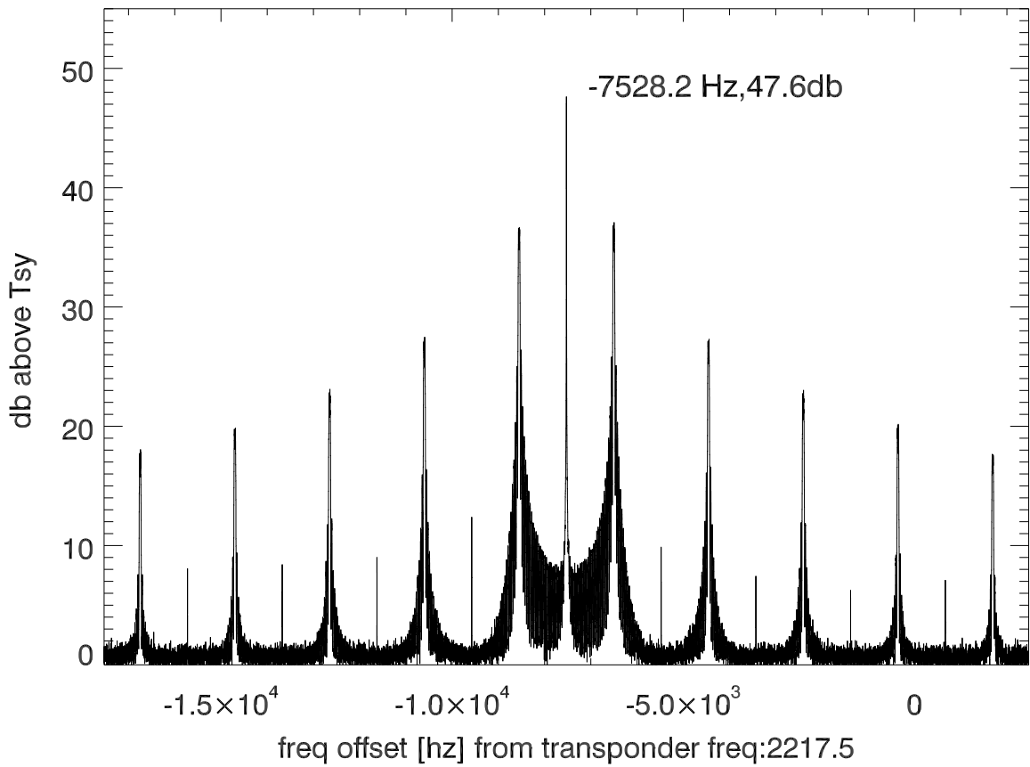
isee3 140610:195915 (UTC) spectra after doppler correction. PolB
