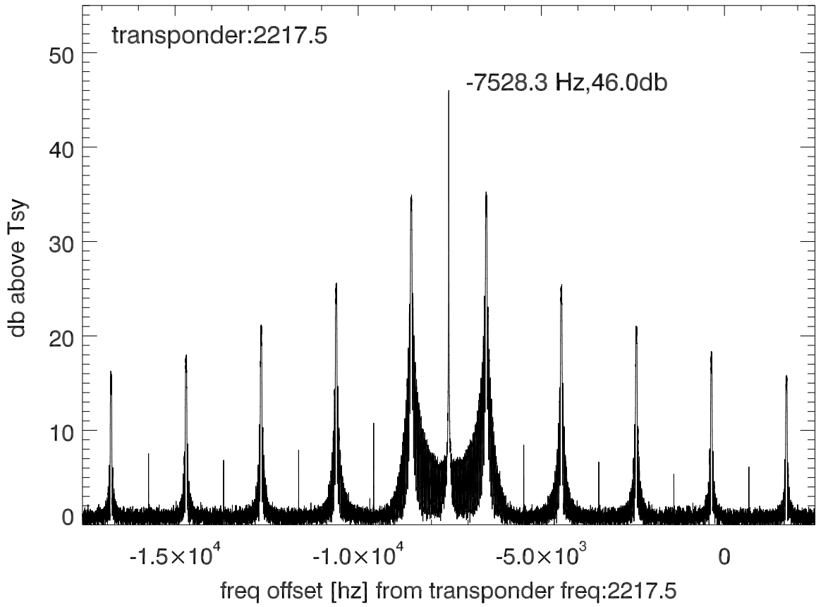
isee3 140610:195915 (UTC) spectra after doppler correction. PolA
