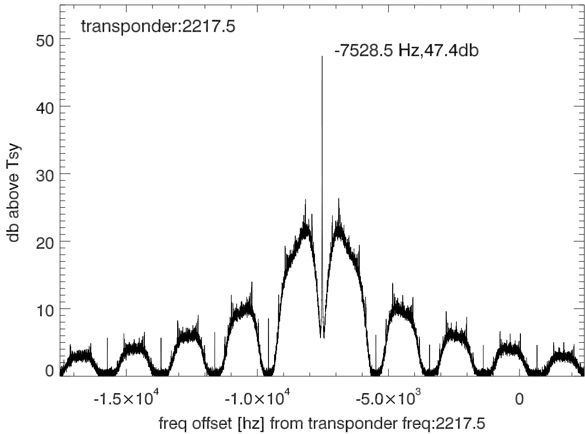
isee3 140610:194607 (UTC) spectra after doppler correction. PolA
