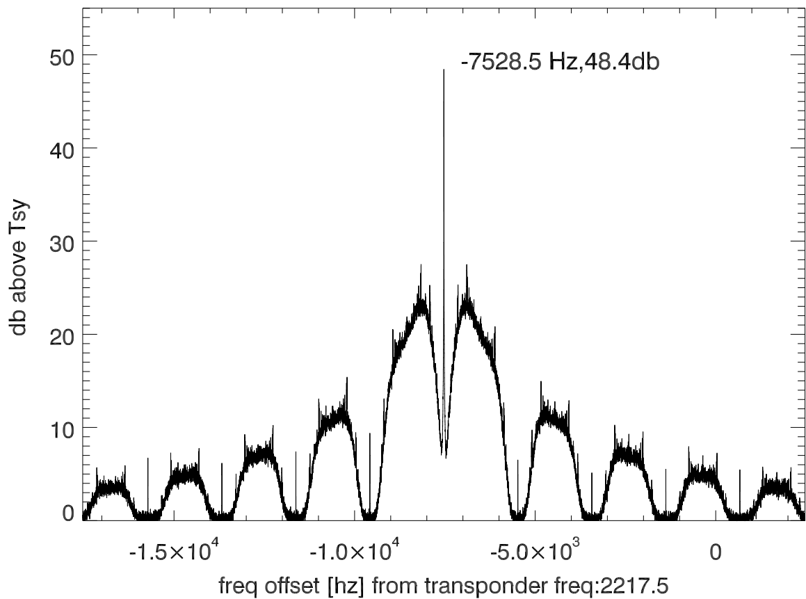
isee3 140610:194607 (UTC) spectra after doppler correction. PolB
