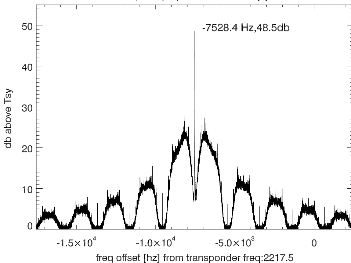
isee3 140610:194145 (UTC) spectra after doppler correction. PolB
