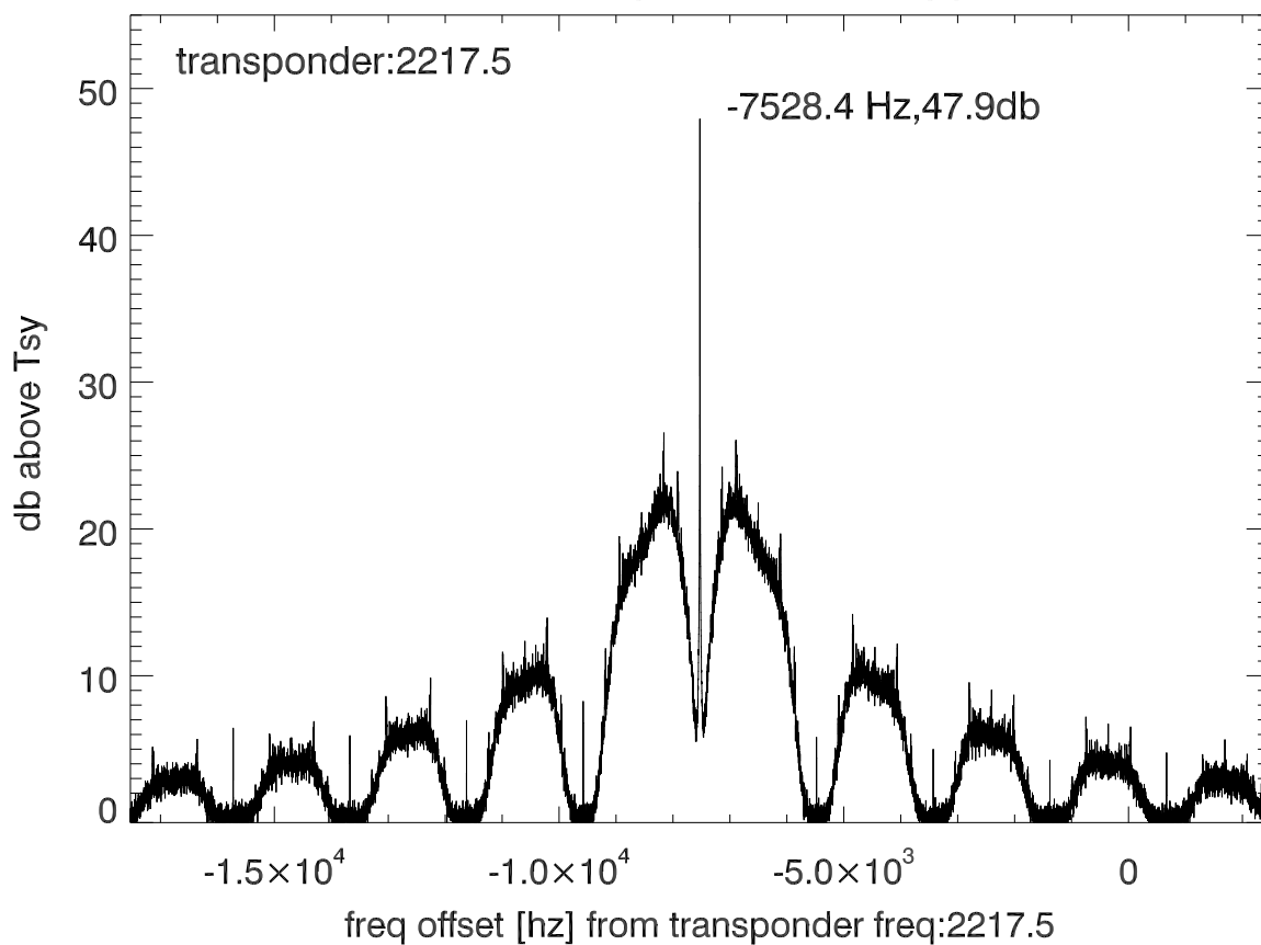
isee3 140610:194145 (UTC) spectra after doppler correction. PolA
