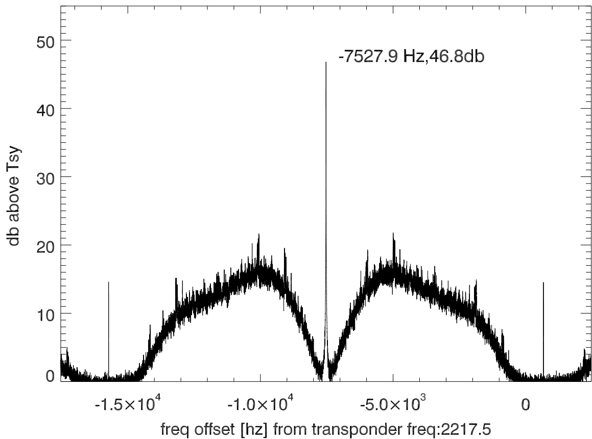
isee3 140610:204139 (UTC) spectra after doppler correction. PoIB
