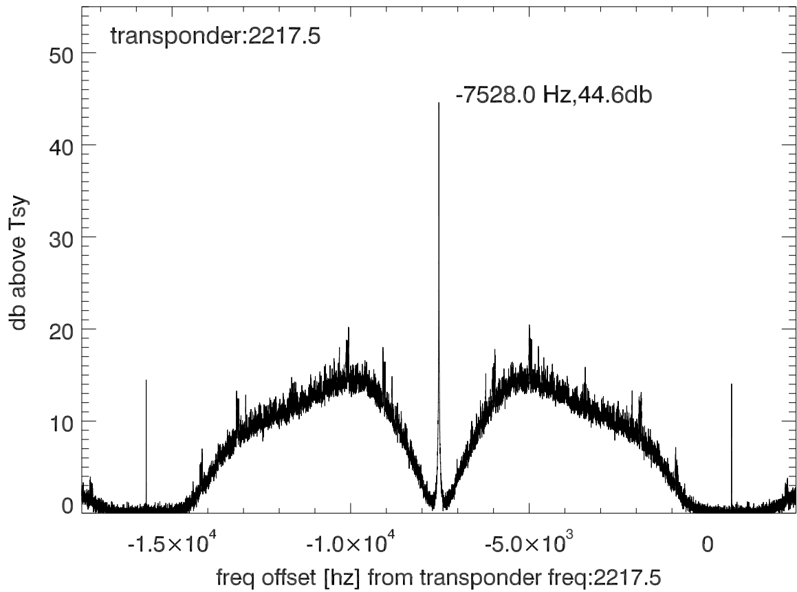
isee3 140610:203344 (UTC) spectra after doppler correction. PolA
