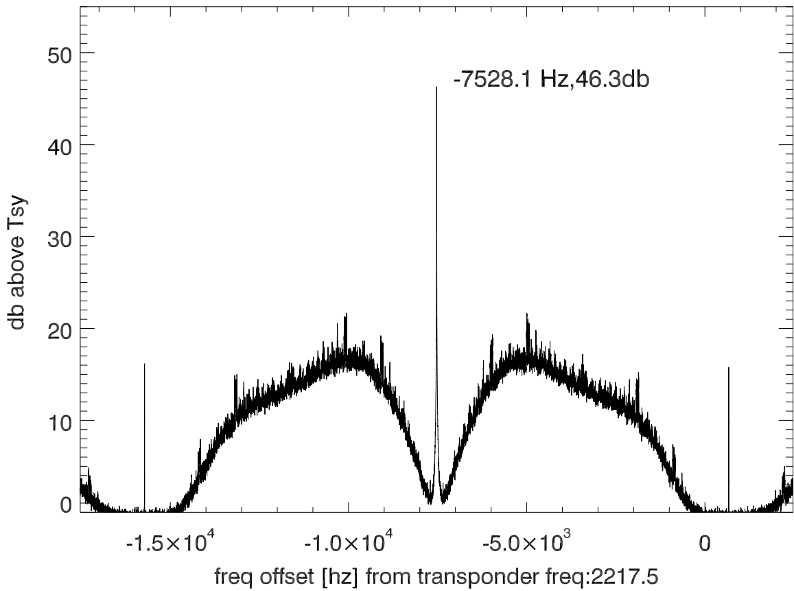
isee3 140610:202227 (UTC) spectra after doppler correction. PoIB
