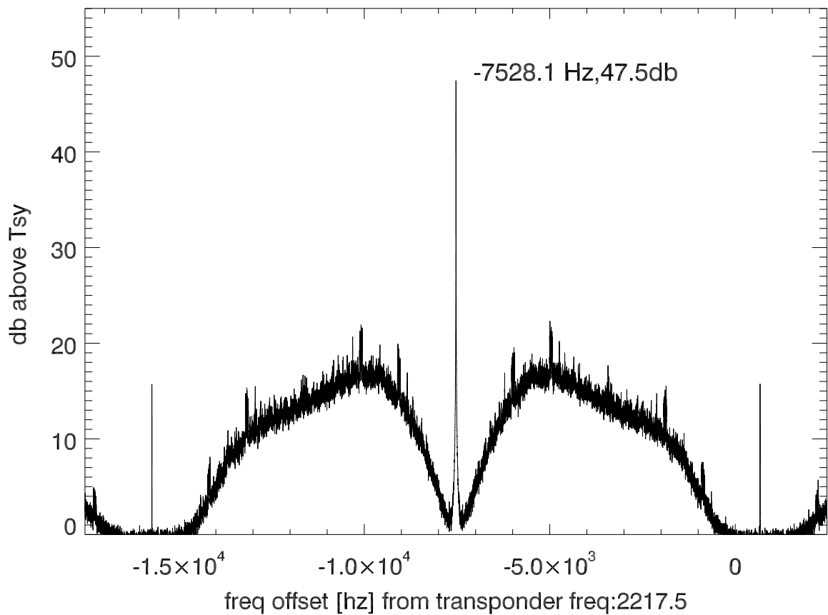
isee3 140610:201310 (UTC) spectra after doppler correction. PolB
