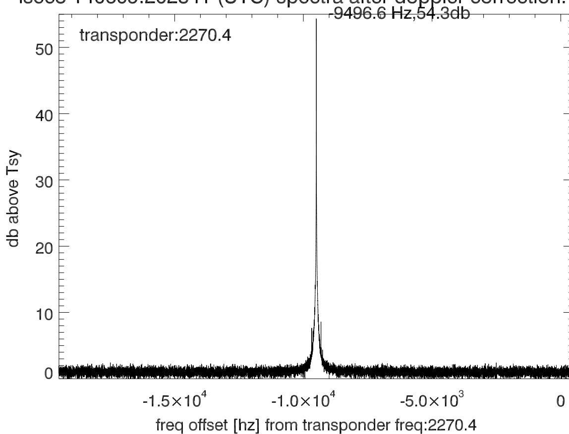
isee3 140609:202841 (UTC) spectra after doppler correction. PolA
