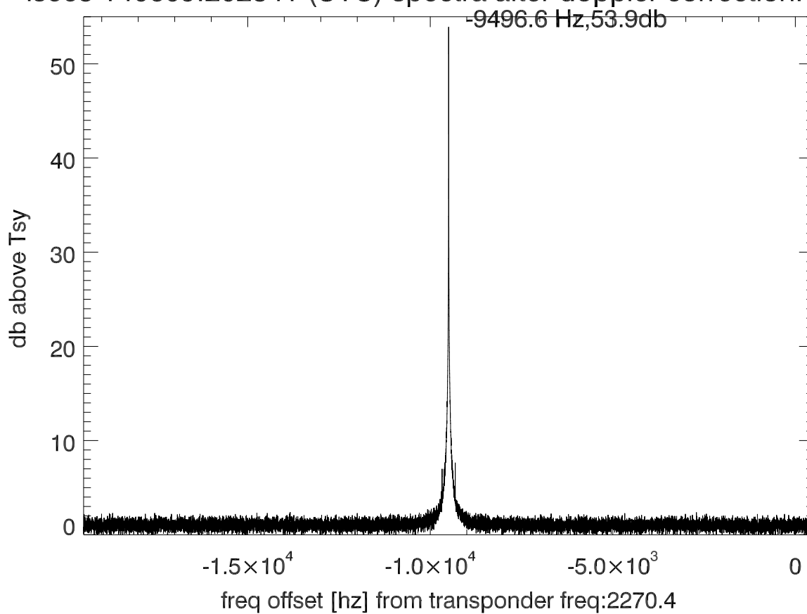
isee3 140609:202841 (UTC) spectra after doppler correction. PolB
