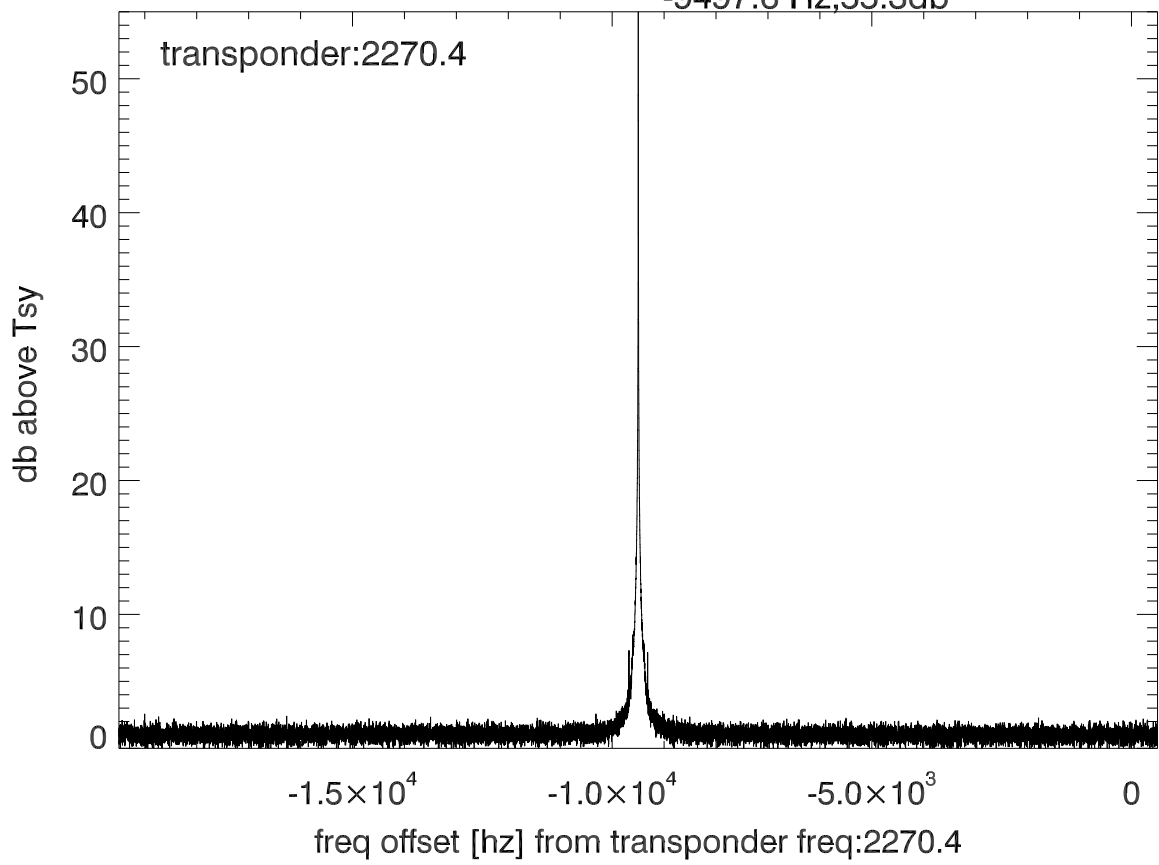
isee3 140609:200020 (UTC) spectra after doppler correction. PolA
